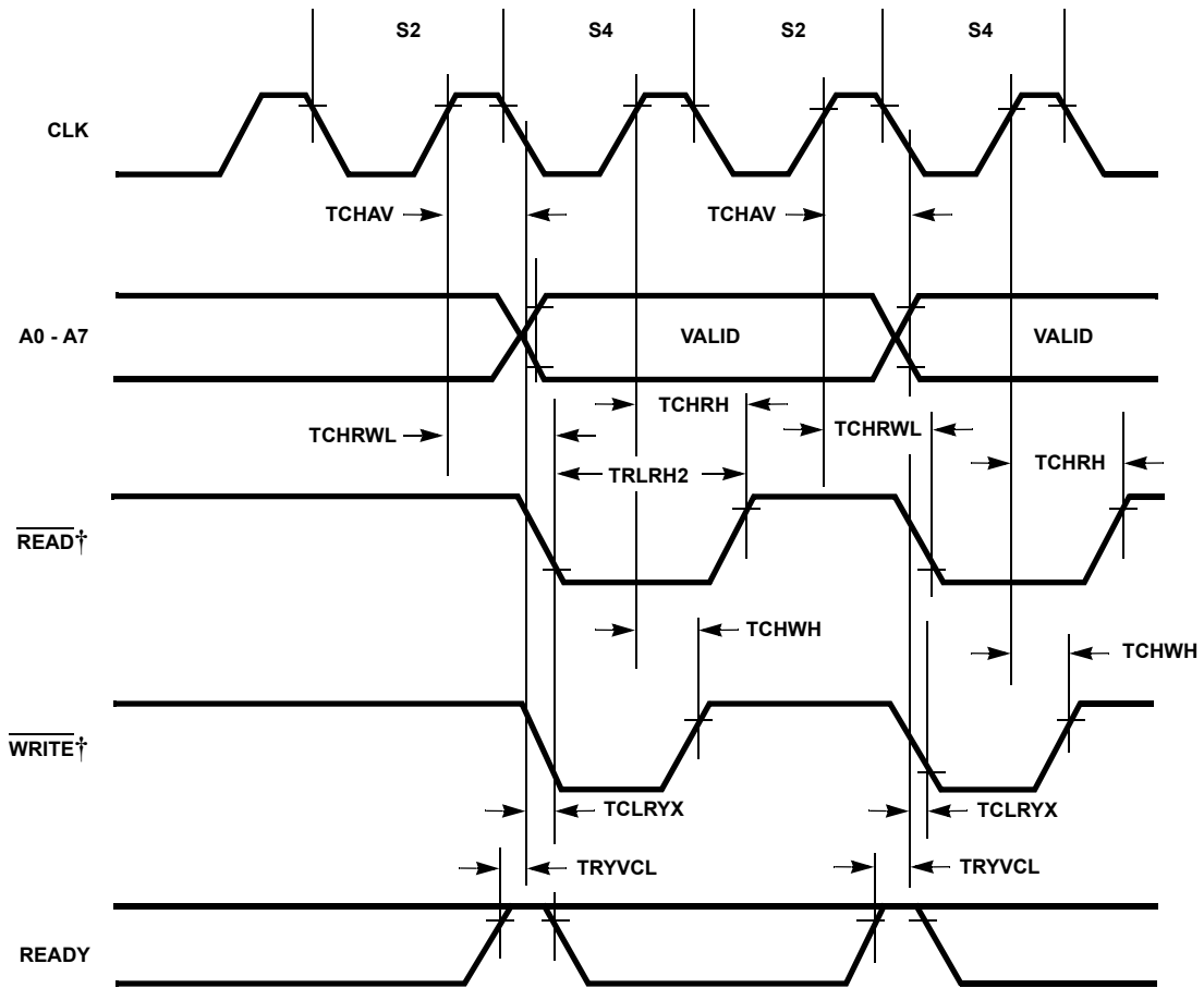
FIGURE 7. COMPRESSED TRANSFER † \overline{\text{READ}} refers to both \overline{\text{IOR}} and \overline{\text{MEMR}} outputs. \overline{\text{WRITE}} refers to both \overline{\text{IOW}} and \overline{\text{MEMW}} outputs.
