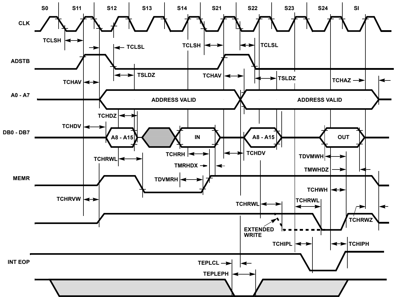
FIGURE 5. MEMORY-TO-MEMORY TRANSFER
