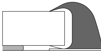
Too much solder Pad geometry too large, not soldered in preferred direction KKE0288-H-E
