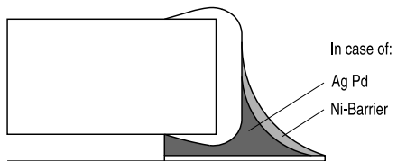
Good solder joint KKE0070-2-E
