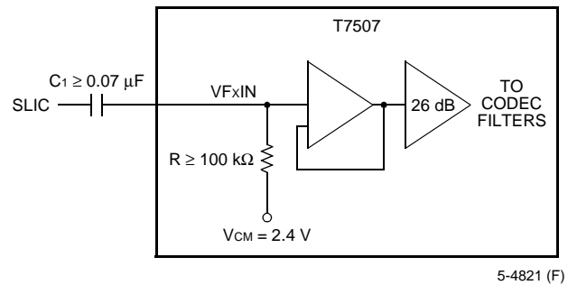
Figure 3. Typical Analog Input Section
