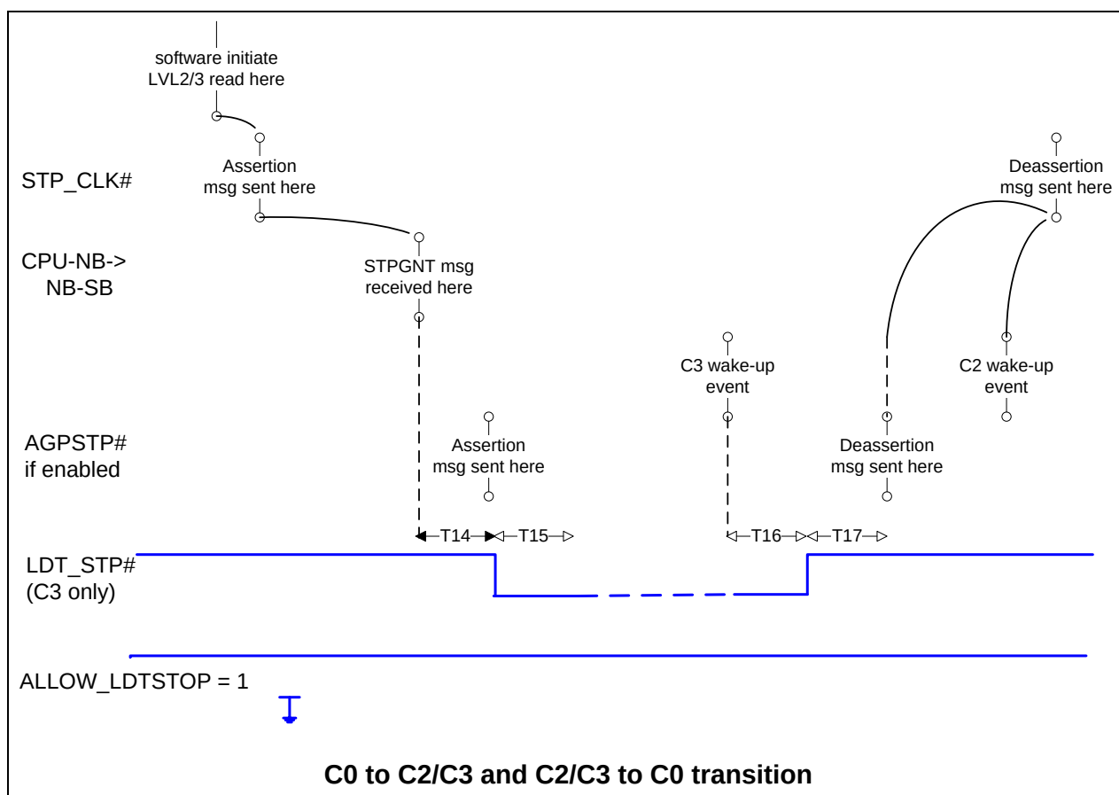
Figure 28. C2/C3-State Timing
