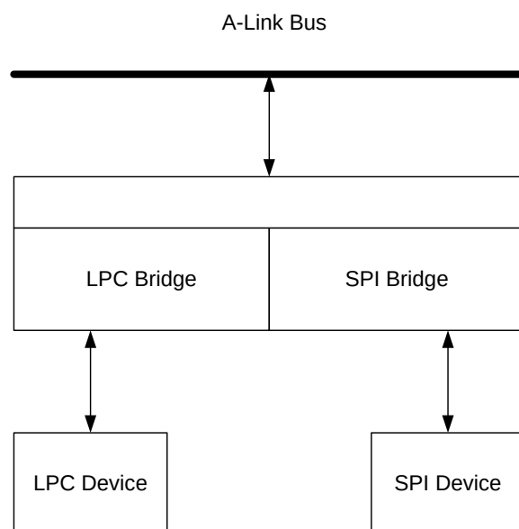
Figure 6. SB810/850 LPC Bus System
