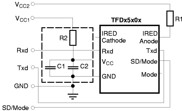
Note: Outlined components are optional depending on the quality of the power supply.
