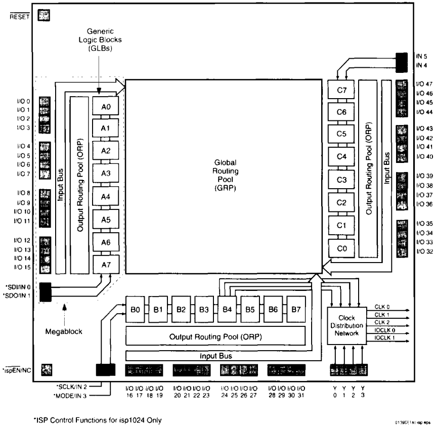
Figure 1. ispLSI and pLSI 1024 Functional Block Diagram
