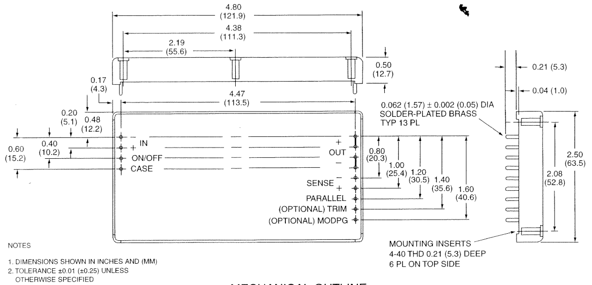
MECHANICAL OUTLINE
