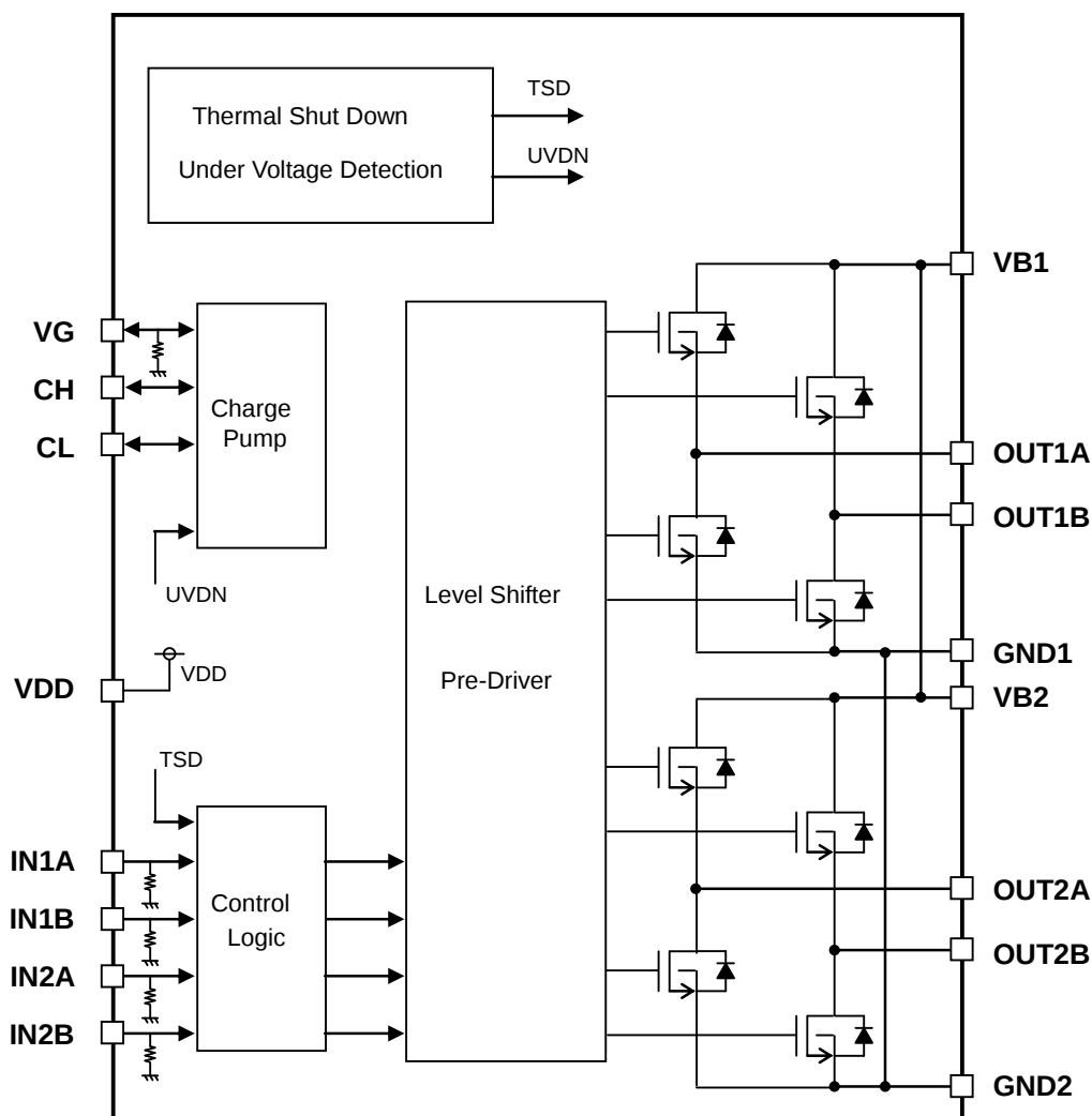
Fig1. Block diagram
