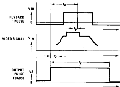
FIGURE 3. Phase Relationships
