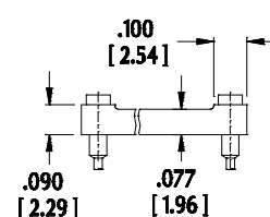
BODY STYLE B
