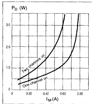
Figure 8. Power dissipation vs. motor current. T_a = 25^{\circ}\text{C} .
