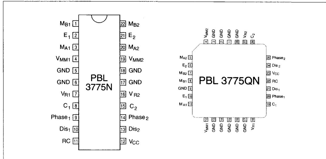
Figure 4. Pin configuration.
