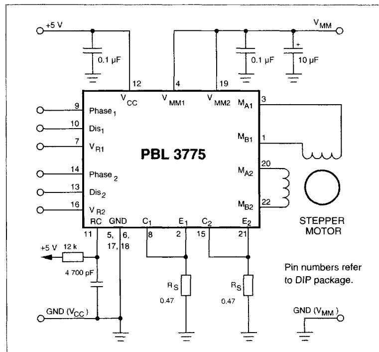
Figure 6. Typical stepper motor driver application with PBL 3775.
