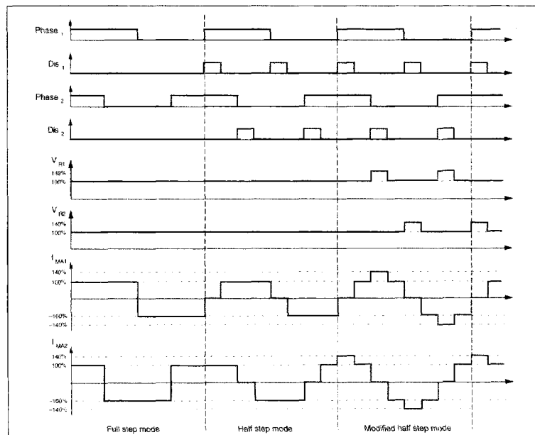
Figure 15. Stepping modes.
