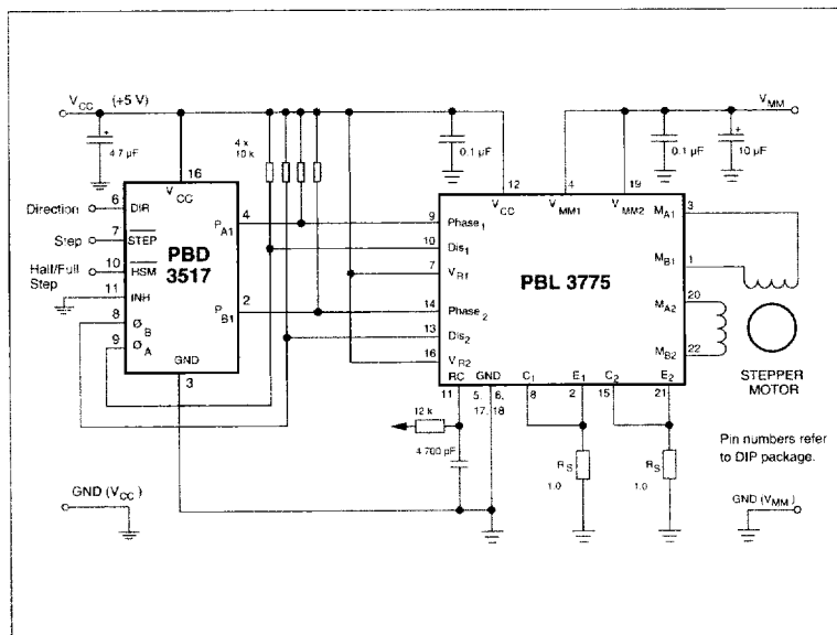
Figure 7. Half stepping system where PBD 3517 is used as controller circuit in order to generate the necessary sequence to the PBL 3775.
