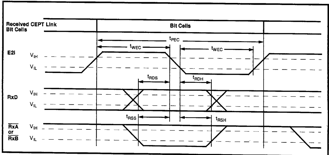
Figure 26 - Receive Timing for CEPT Link
