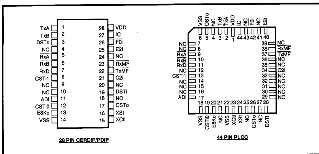
Figure 2 - Pin Connections
