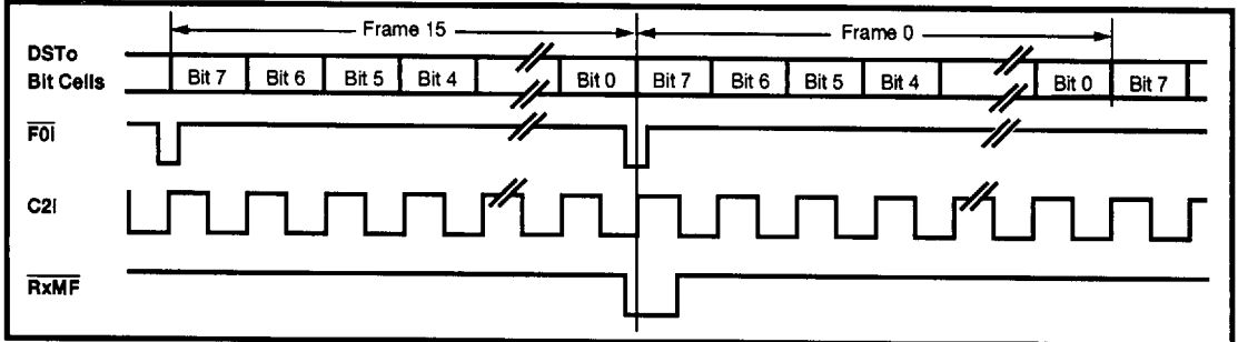
Figure 19 - Functional Timing for Receive Multiframe Clocks
