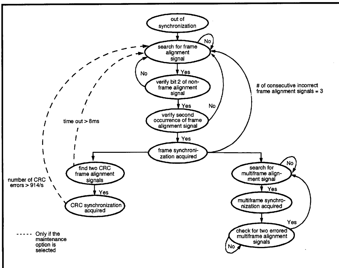
Figure 13 - Synchronization State Diagram
