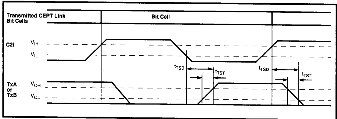
Figure 25 - Transmit Timing for CEPT Link
