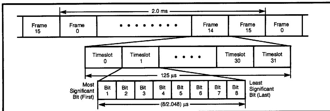
Figure 3 - CEPT Link Frame & Multiframe Format
