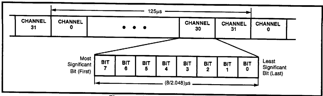
Figure 7 - ST-BUS Stream Format
