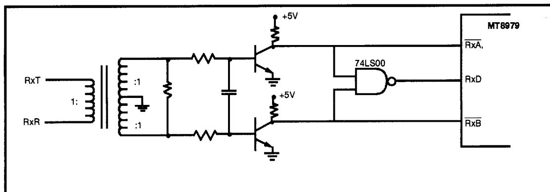
Figure 15 - Typical Bipolar Line Receiver
