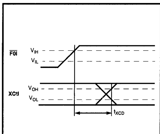
Figure 22 - XCtl Timing
