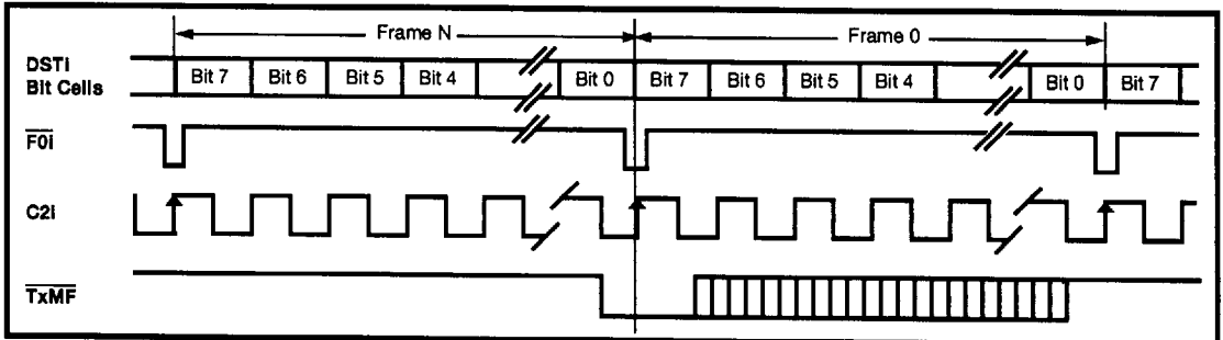
Figure 20 - Functional Timing for Transmit Multiframe Clock
