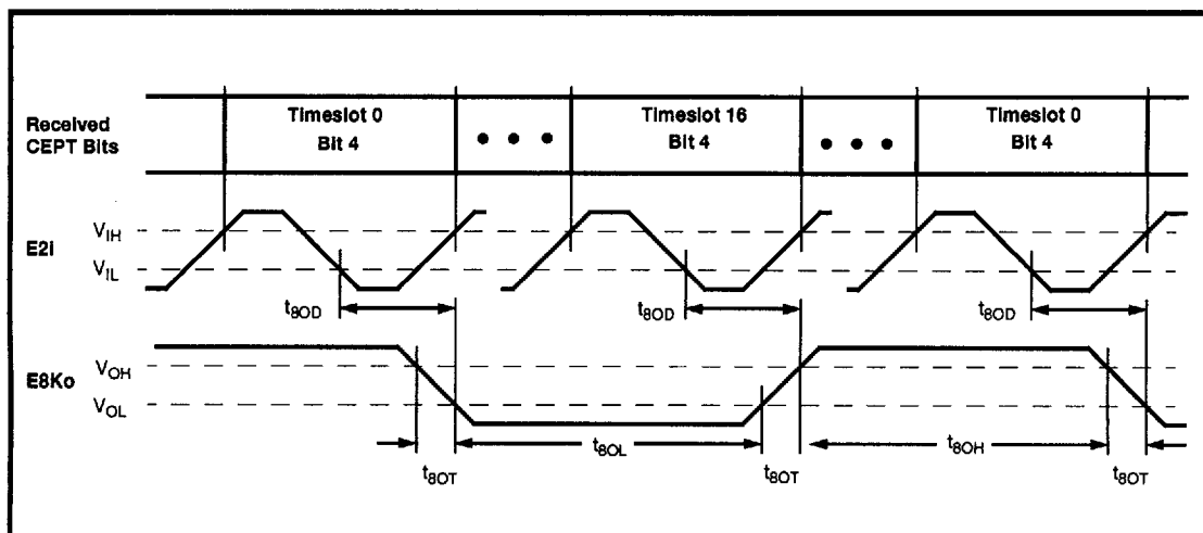
Figure 24 - E8Ko Timing
