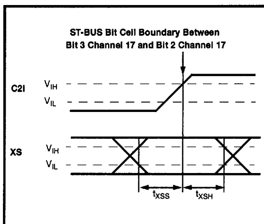
Figure 23 - XS Timing
