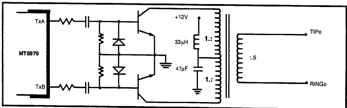
Figure 14 - Bipolar Line Driver
