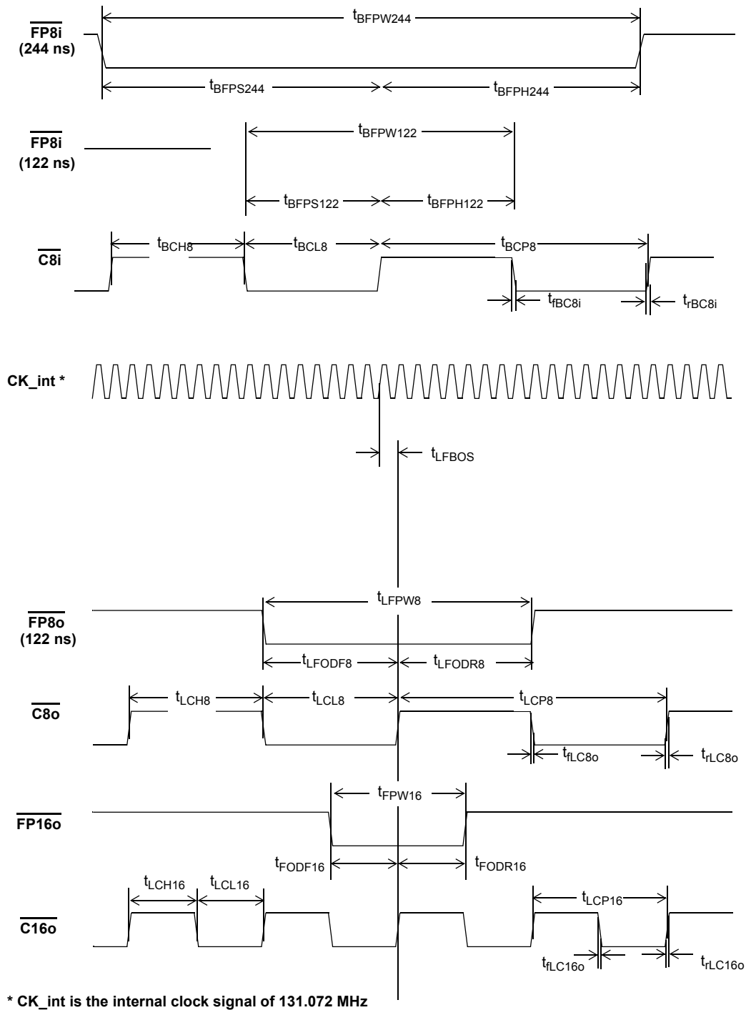
Figure 19 - Backplane and Local Clock Timing Diagram for ST-BUS
