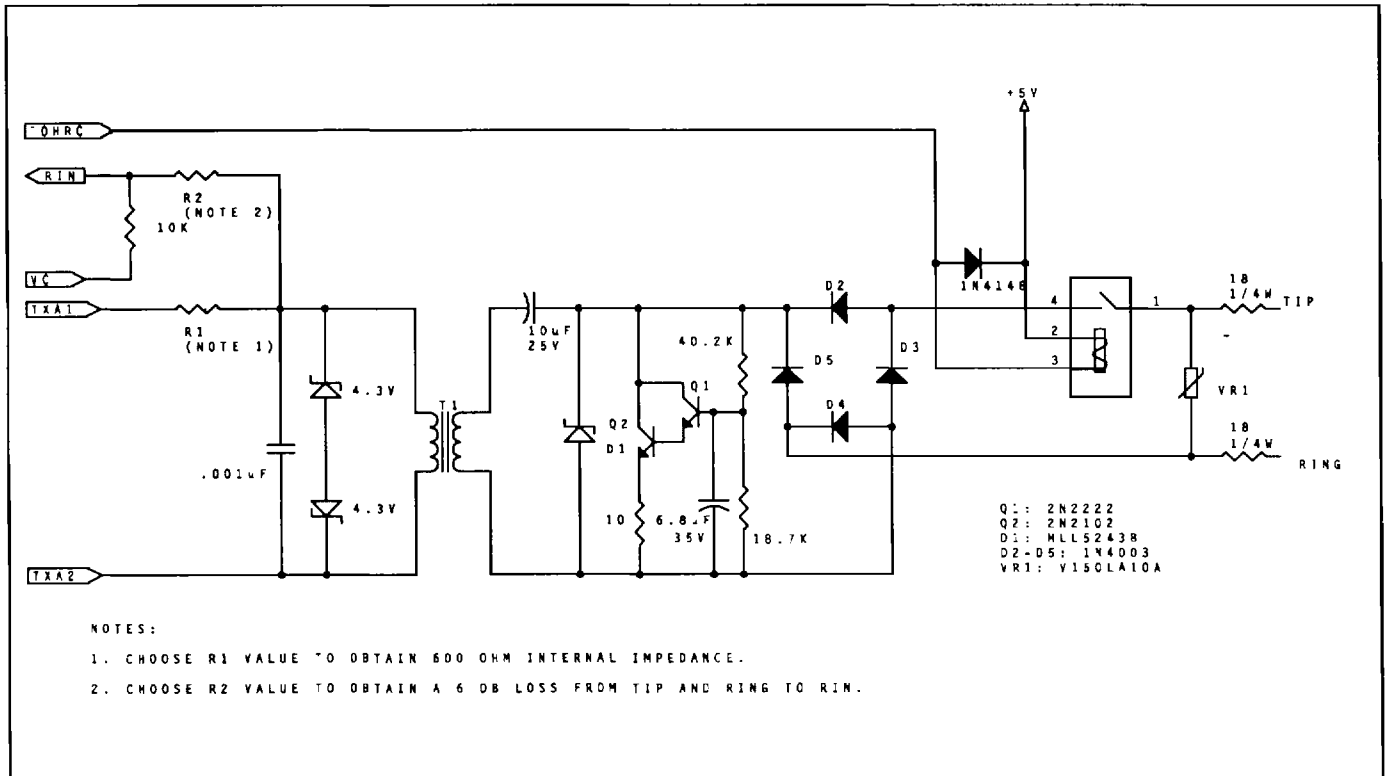
Figure 8-4. Typical Line Interface
