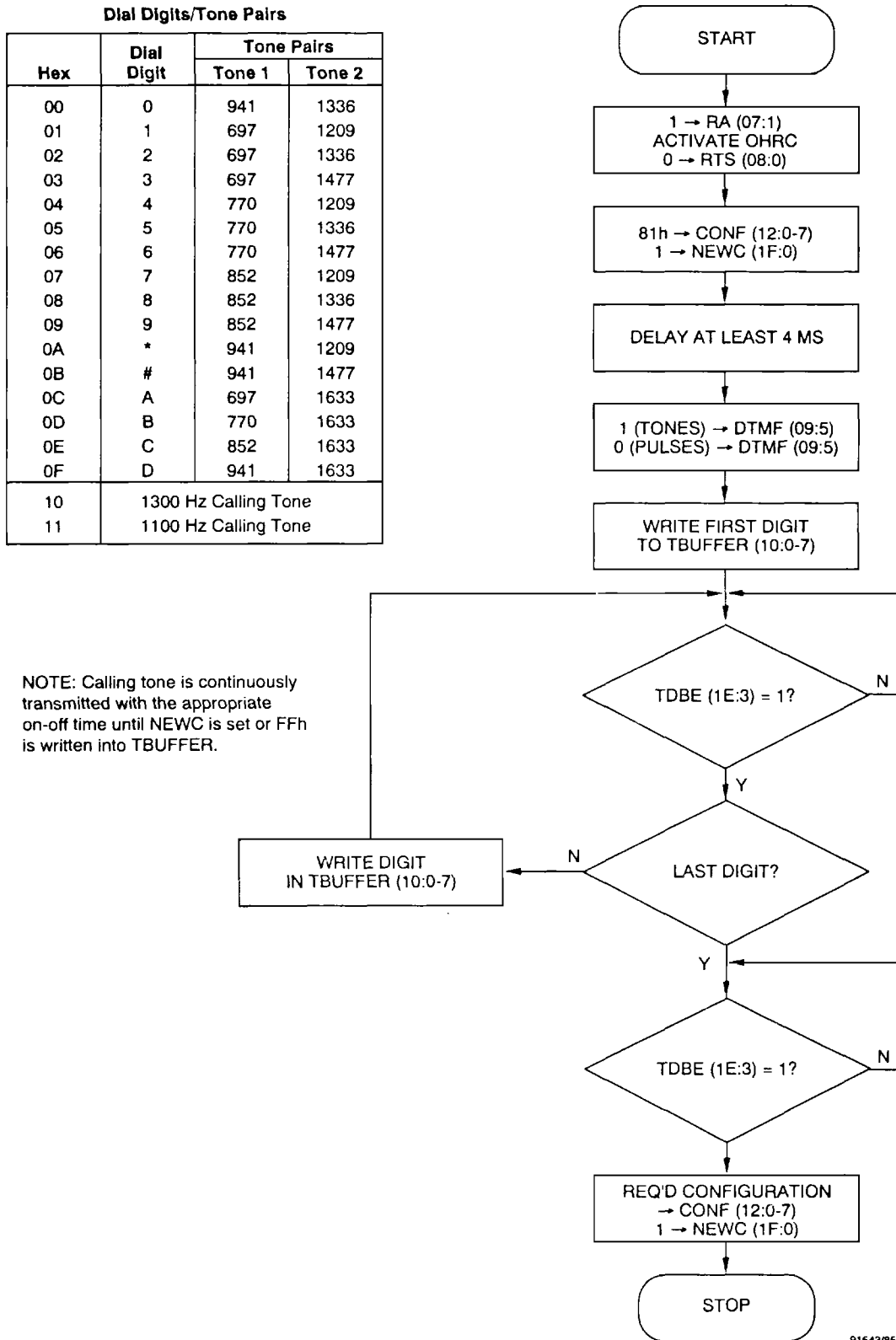
Figure 3-2. Auto Dial Sequence and Dial Digits
