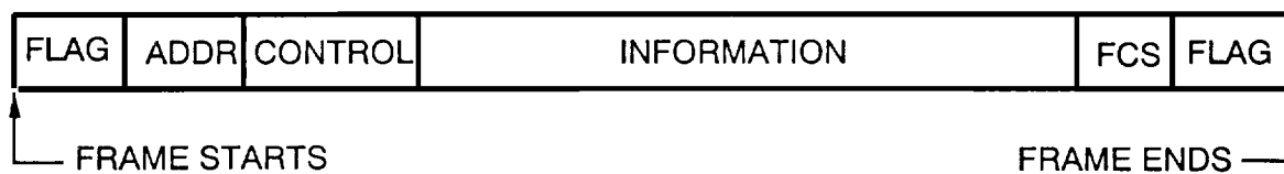
Figure 5-1. HDLC Frame
