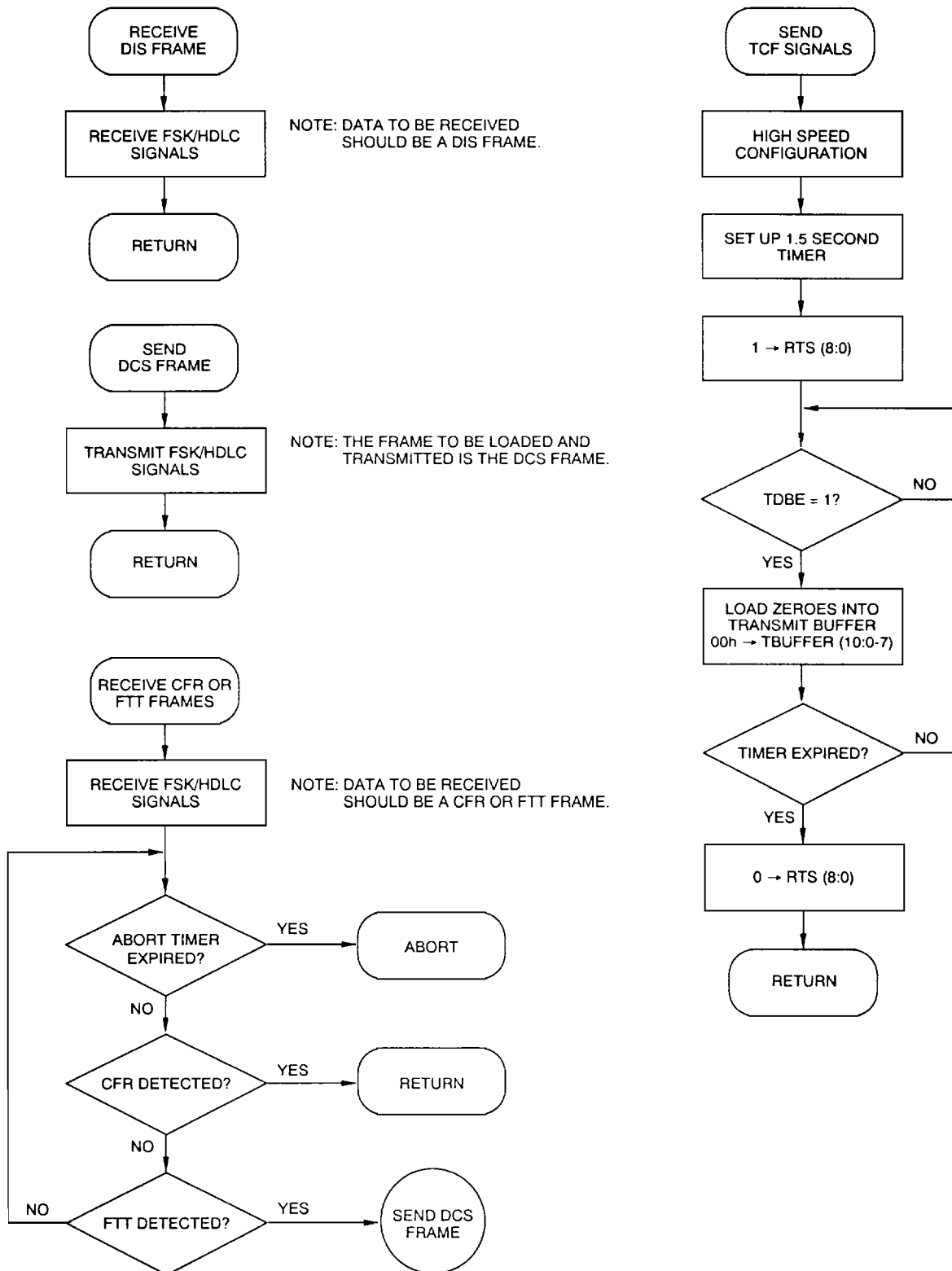
Figure 9-5. Originating a Fax Call - Phase B
