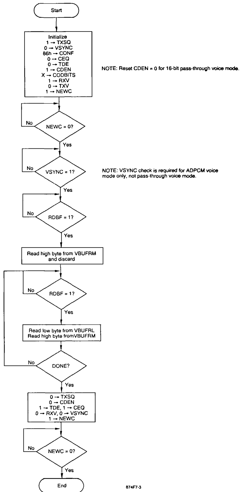
Figure 7-3. Rx-Coder Operation
