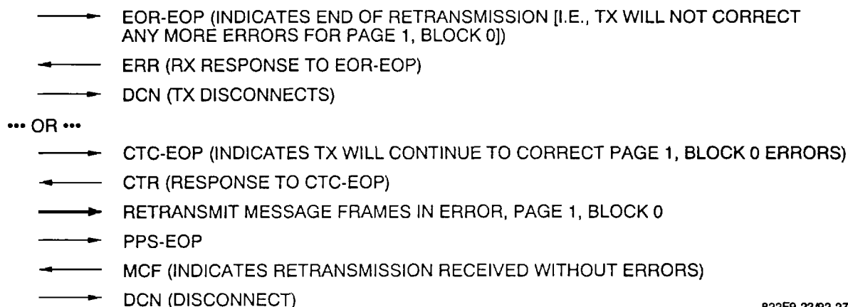
Figure 9-23. ECM Message Protocol Example
