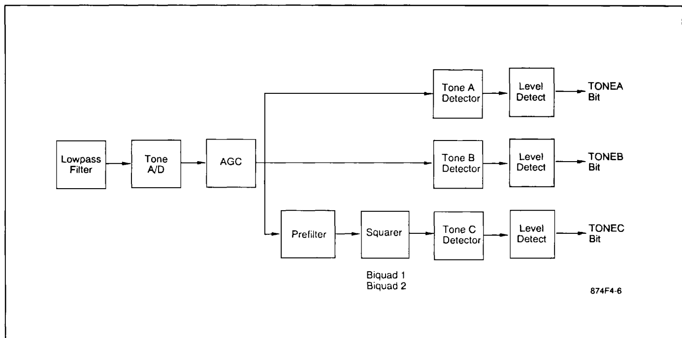
Figure 4-6. Tone Detectors
