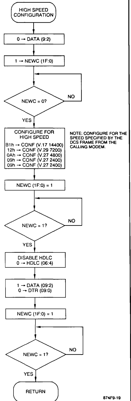
Figure 9-19. High Speed Configuration Routine
