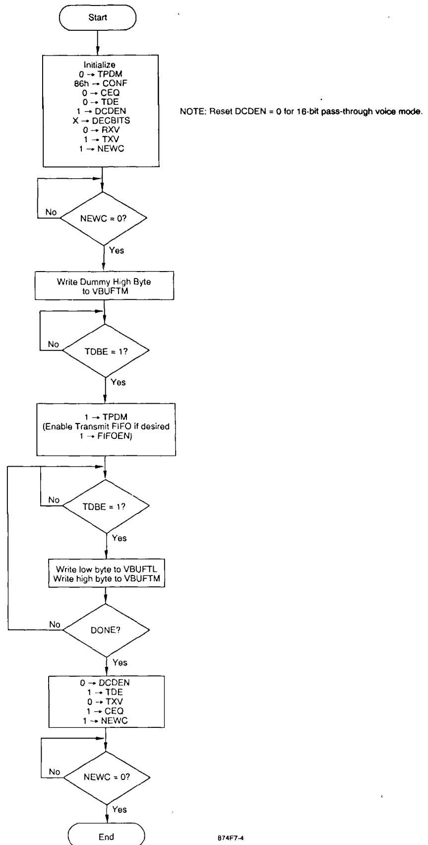
Figure 7-4. Tx-Decoder Operation
