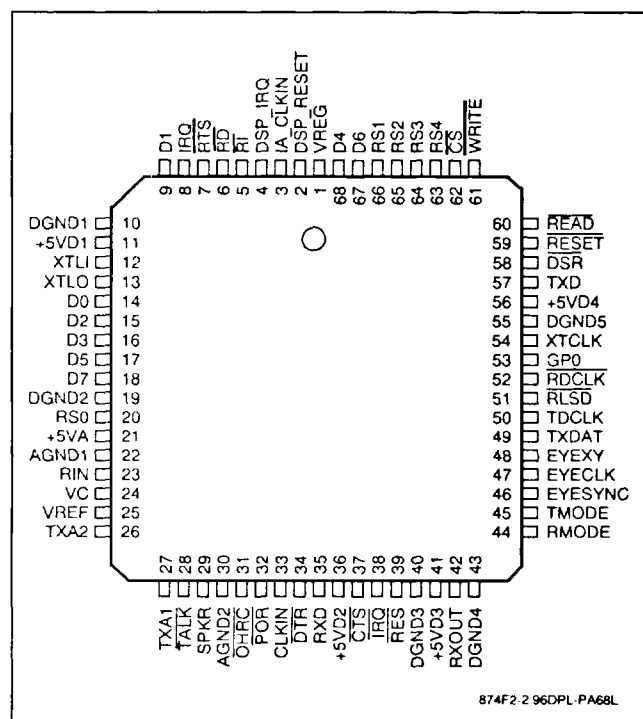
Figure 2-2. Pin Assignments- 68-Pin PLCC
