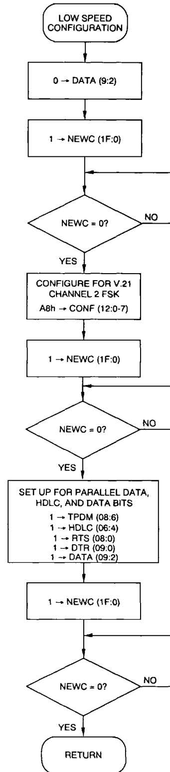
Figure 9-15. Low Speed Configuration Routine
