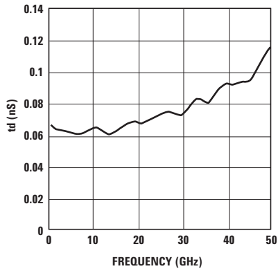
Figure 4. Group Delay.
