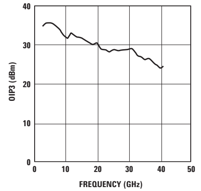
Figure 6. Output IP3.
