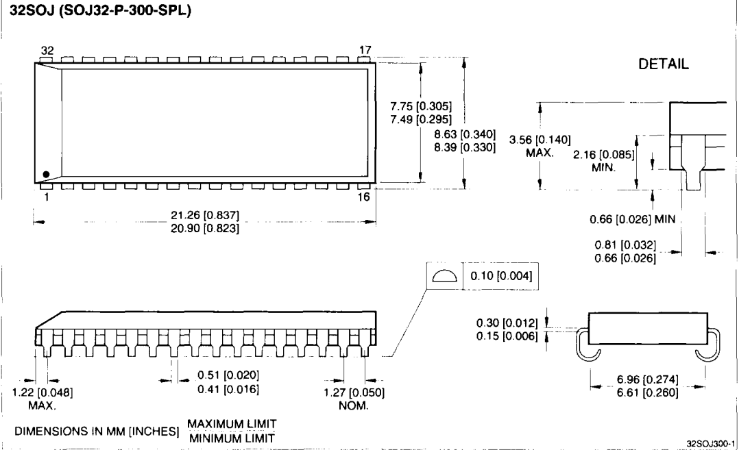
32-pin, 300-mil SOJ (Preliminary)
