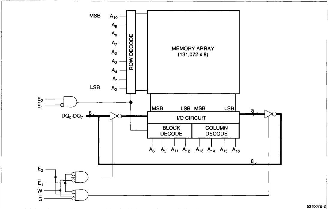
Figure 2. LH521007B Block Diagram
