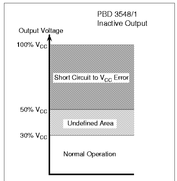
Figure 6. Error state vs. output voltage, inactive output ( 2.0V \leq V_{IN} \leq V_{CC} , 5V \leq V_{CC} \leq 40V and -40^\circ C < T_J < +100^\circ C ).
