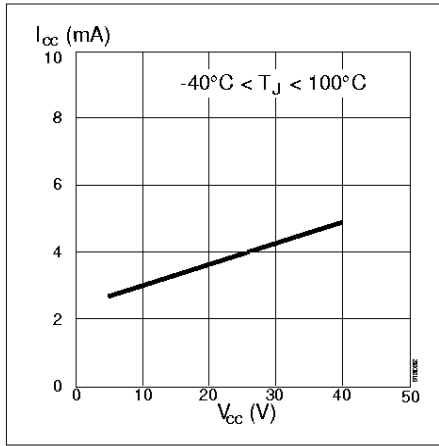
Figure 7. Current consumption vs. supply voltage at 2\text{ V} \leq V_{in} \leq V_{CC} . (Inactive output)
