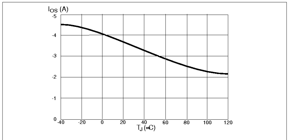
Figure 14. Output current shut-down vs. chip temperature. 5\text{ V} \leq V_{CC} \leq 40\text{ V} .
