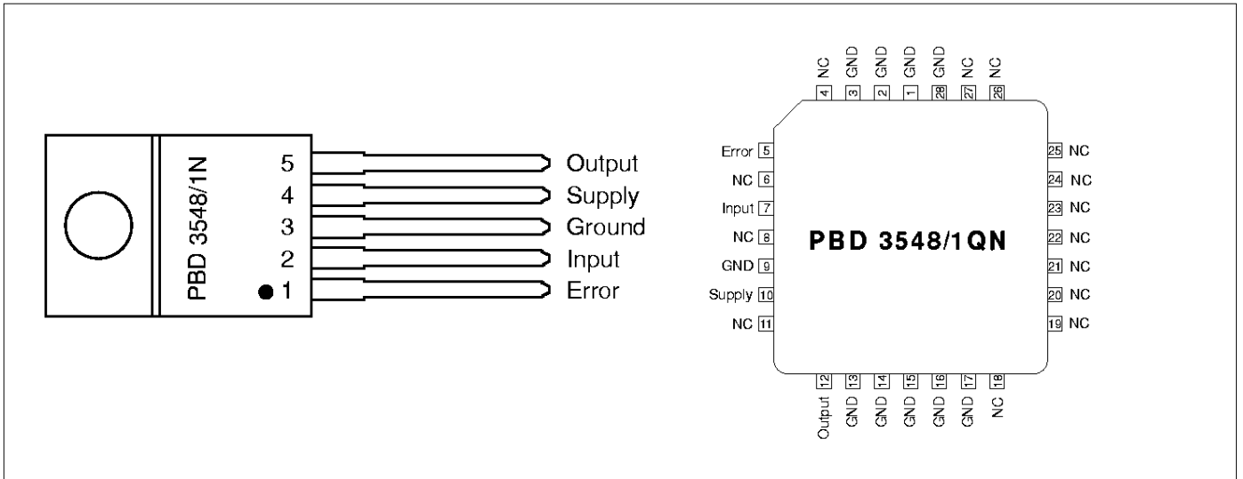
Figure 4. Pin descriptions.
