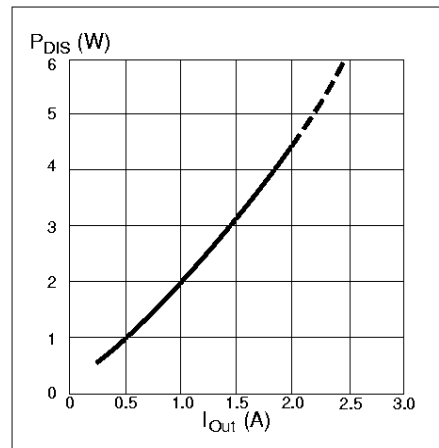
Figure 13. Power dissipation vs. output current.
