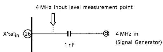
Fig.6 X'tal External Input Reference Application
