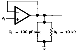
FIGURE 1. UNITY-GAIN AMPLIFIER
