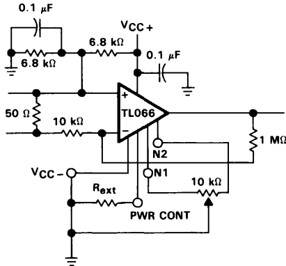
FIGURE 28. AC AMPLIFIER
