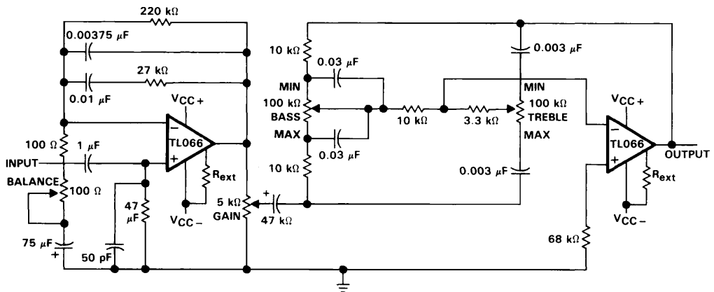
FIGURE 30. IC PREAMPLIFIER
