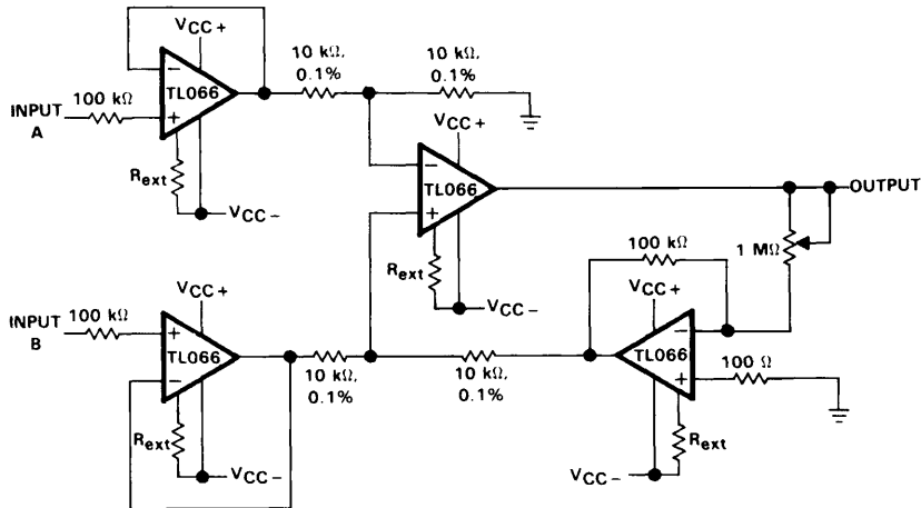
FIGURE 26. INSTRUMENTATION AMPLIFIER
