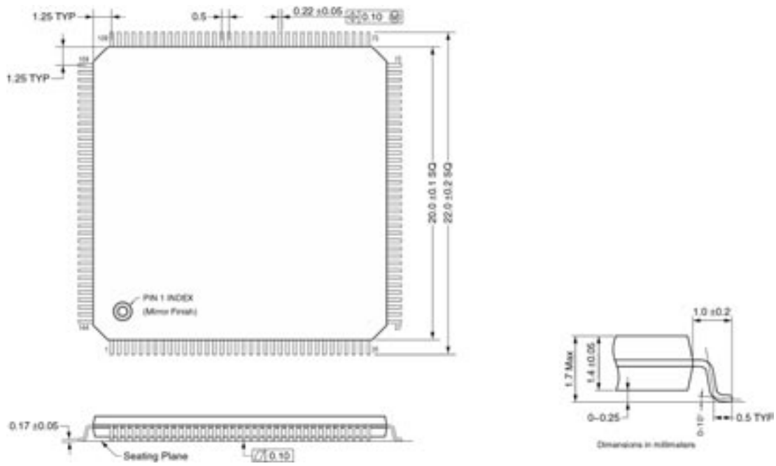
Figure 4. LQFP144-P-2020-0.50-K
