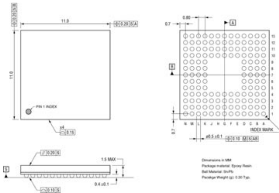
Figure 3. P-LFBGA144-1111-0.80
