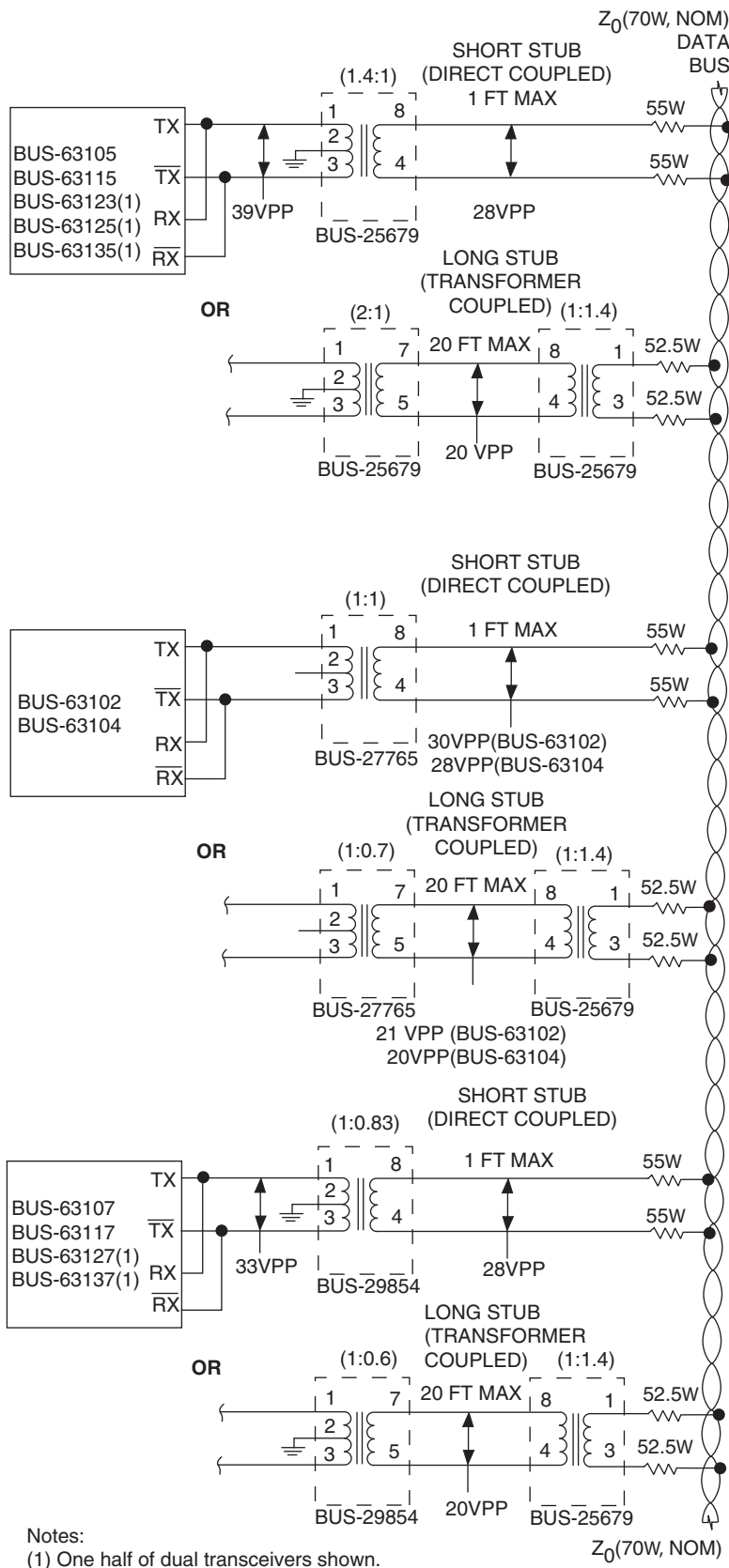
FIGURE 2. BUS COUPLING CONFIGURATIONS
