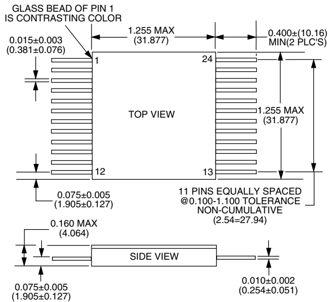
FIGURE 7. BUS-63112 AND BUS-63114 MECHANICAL OUTLINE 24-PIN SQUARE PACKAGE
