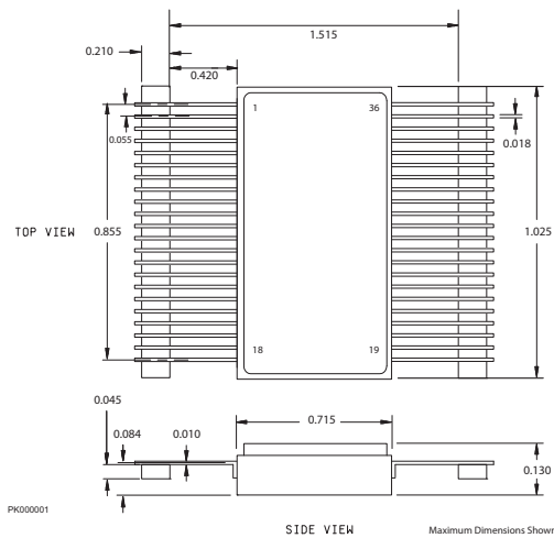
FIGURE 12. BUS-63123 MECHANICAL OUTLINE 36-PIN FLAT PACK (0.050" PITCH)
