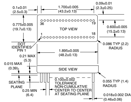
FIGURE 10. BUS-63125, BUS-63127, BUS-63135, AND BUS-63137 MECHANICAL OUTLINE 36-PIN DDIP
