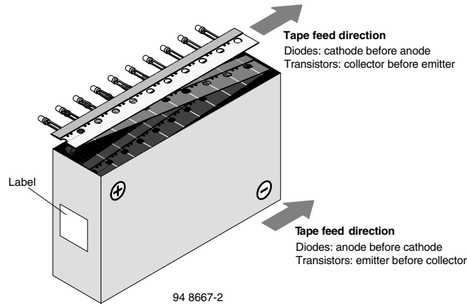
Fig. 24 - Tape Direction
