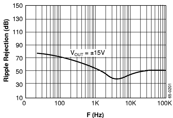
Figure 1. Ripple Rejection vs. Frequency
