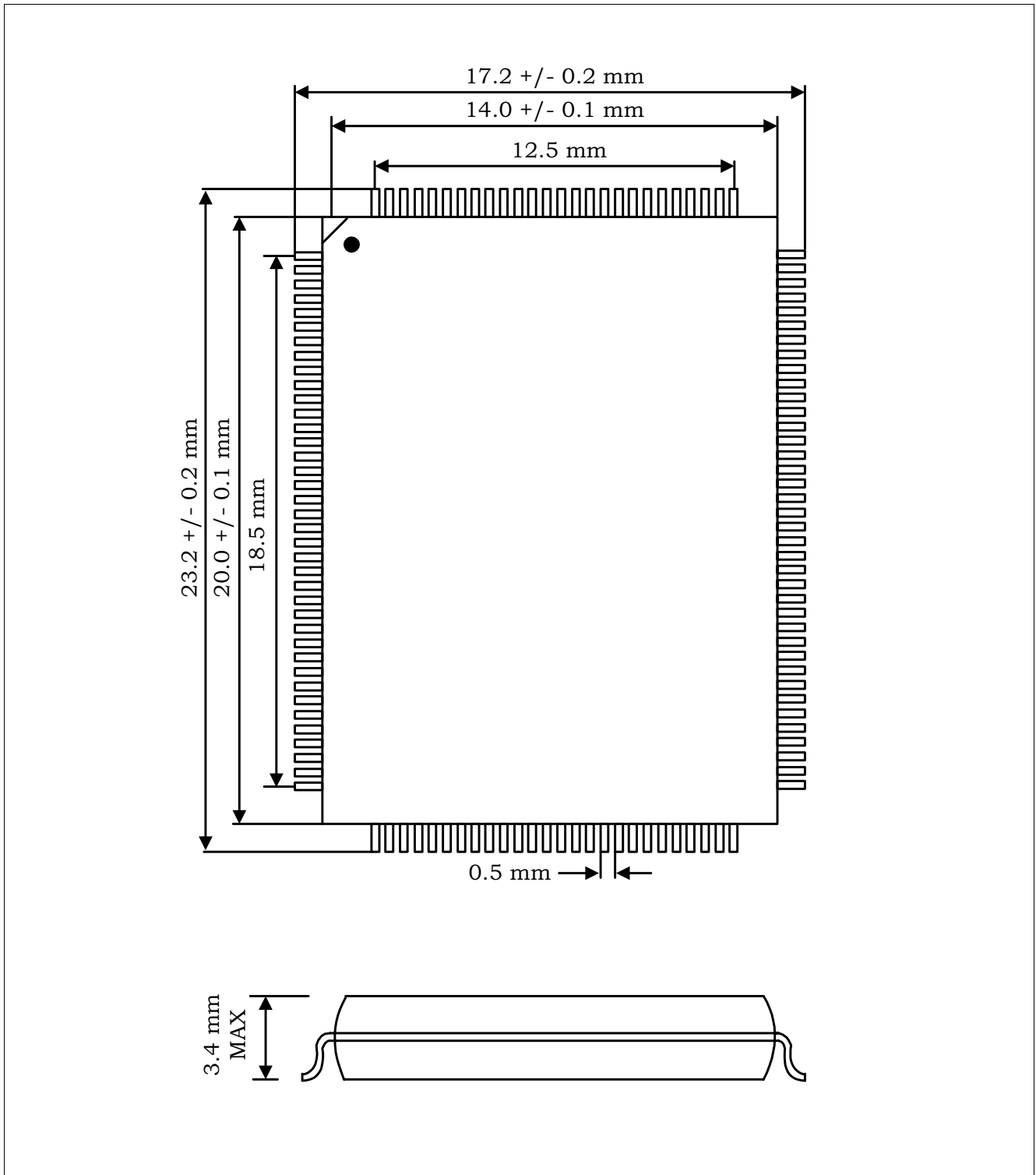
Figure 15 128 PQFP packaging for ADM6992/X
