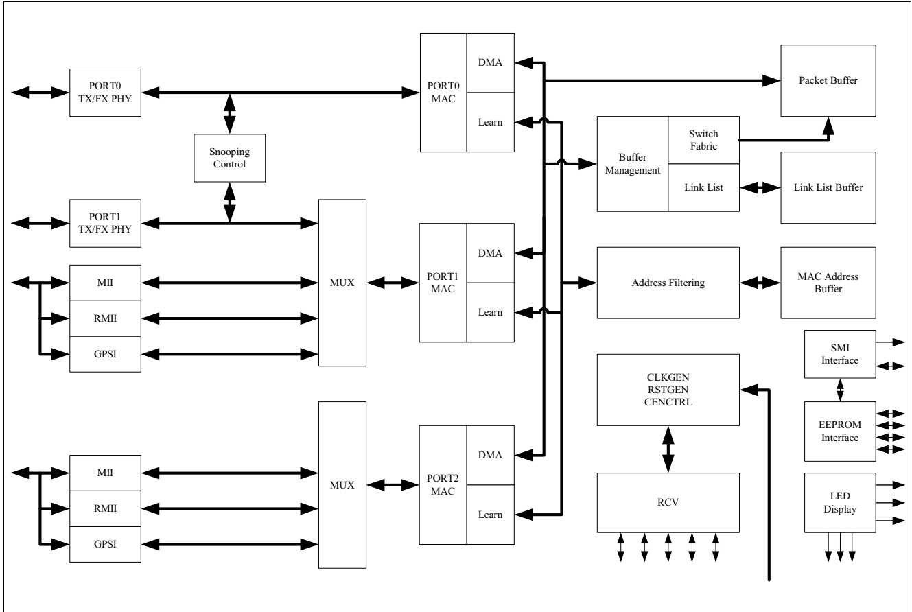
Figure 1 ADM6992/X Block Diagram
