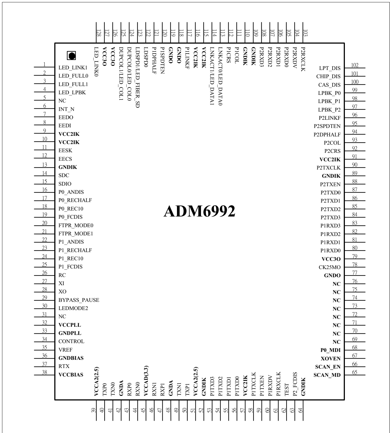
Figure 2 ADM6992/X 64-Pin Assignment
