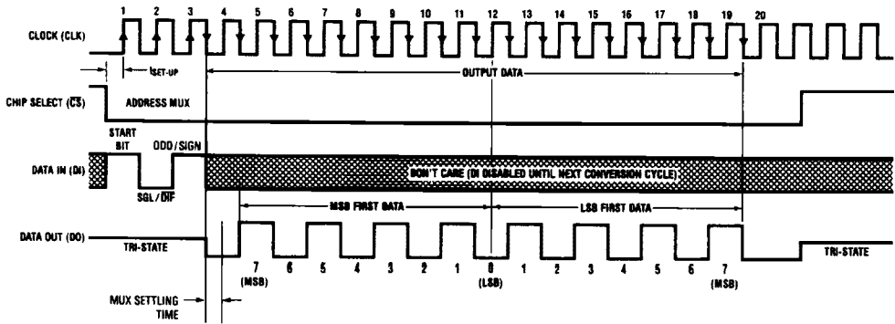
ADC0832 Timing
