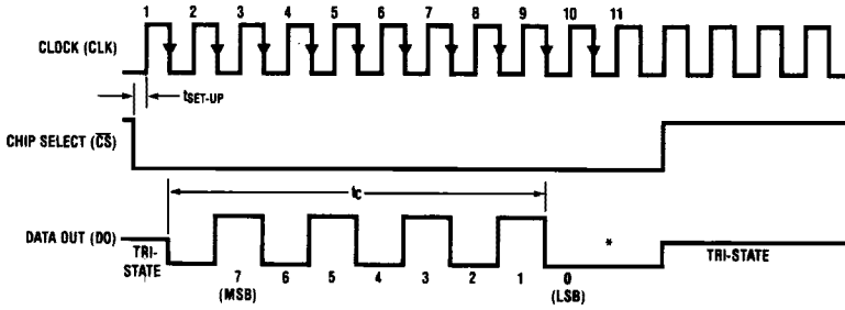
ADC0831 Timing
