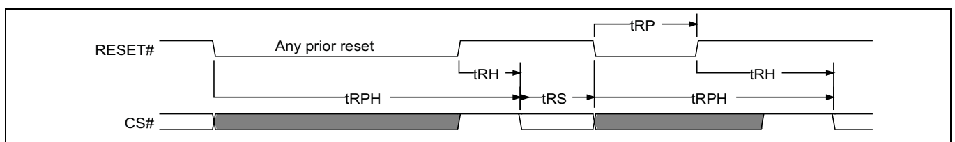
Figure 29 Hardware reset
