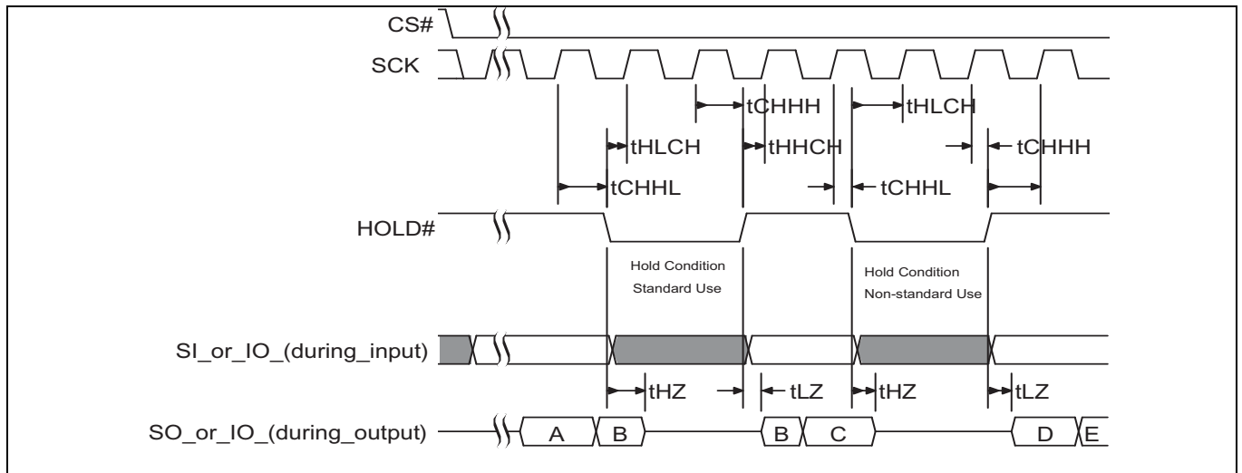
Figure 34 Hold timing
