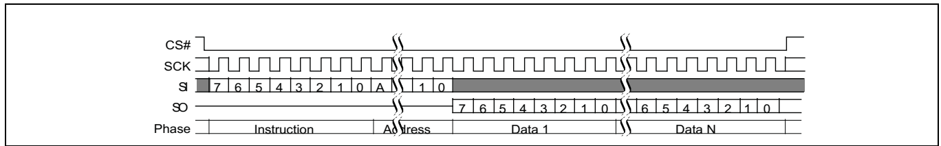
Figure 70 Read command sequence (READ 03h or 13h)
