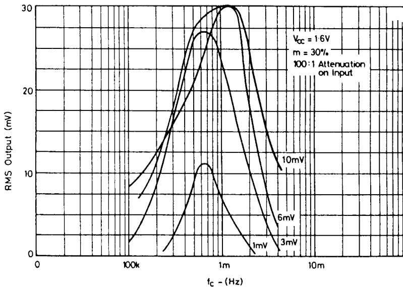
Frequency response of the ZN414Z
