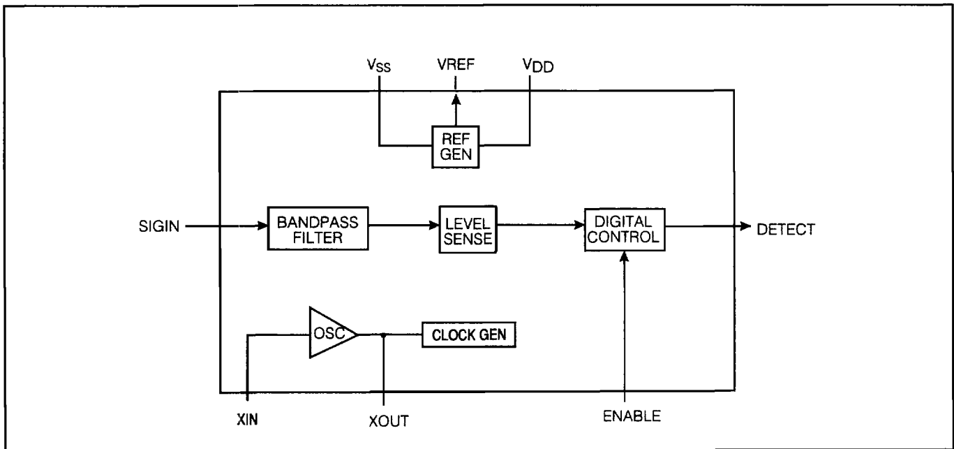
Figure 2 Block Diagram
