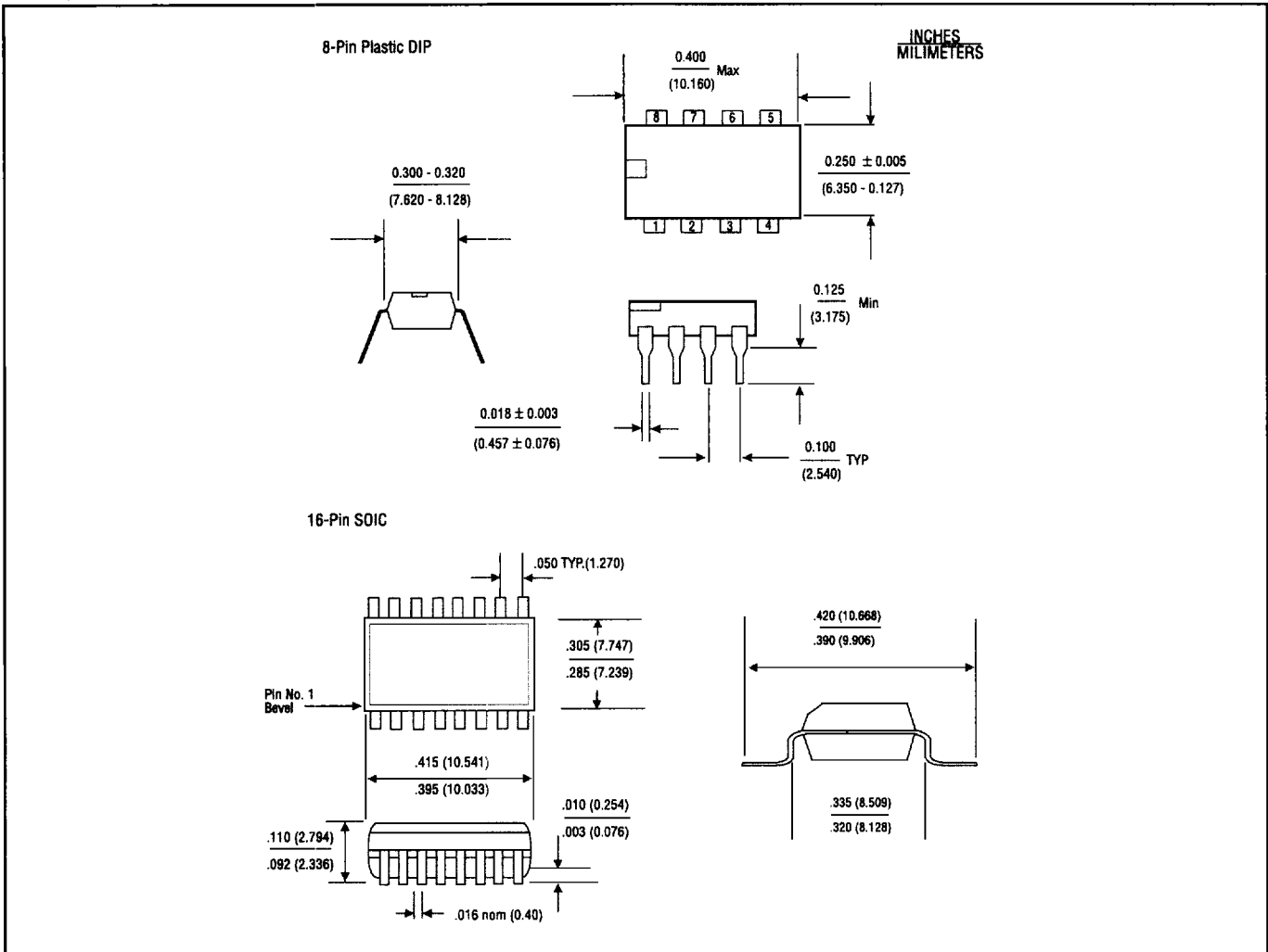
Figure 6 Package Dimensions
