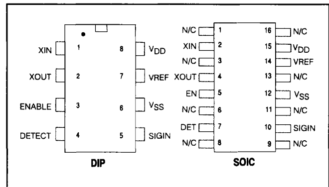
Figure 1 Pin Diagram
