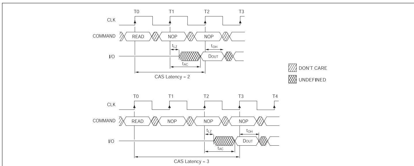
FIGURE 4 – CAS LATENCY
