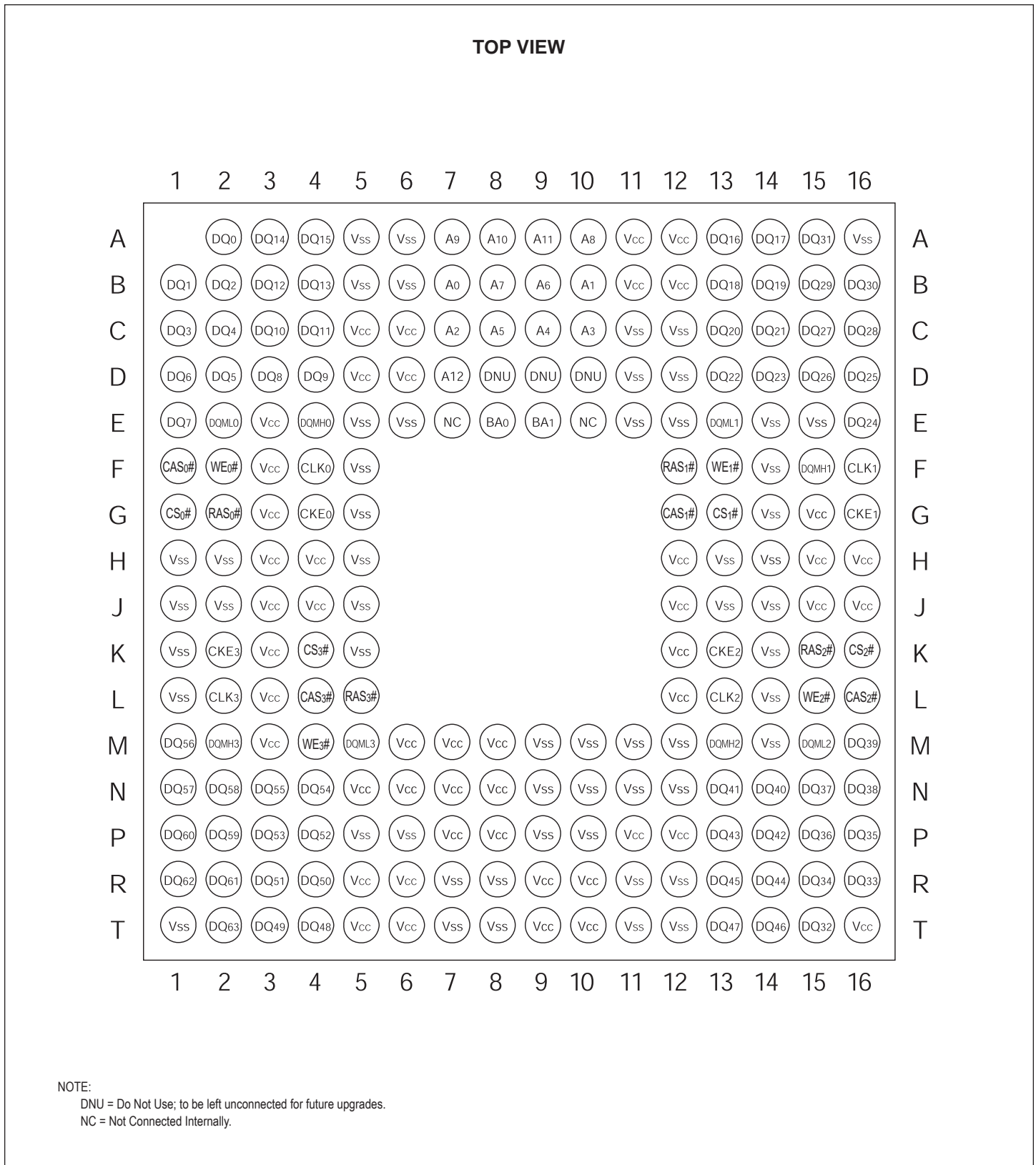
FIGURE 1 – PIN CONFIGURATION
