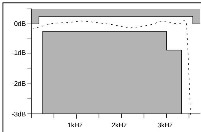
Figure 5 - RX Low-Pass Filter Response
