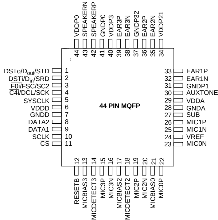
Figure 2 - Pin Description
