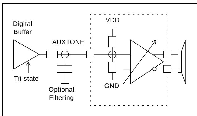
Figure 7 - AUXTONE Circuitry
