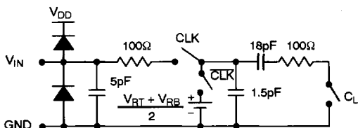
Figure 4. Equivalent Input Circuit
