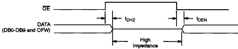
Figure 3. Three-State Timing Diagram
