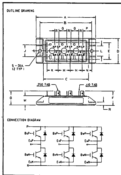
IEF260A2 Outline Drawing
