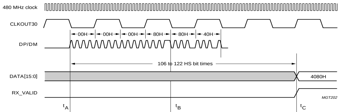
Fig 20. HS receive path delay.
