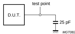
Fig 32. Load for VM, VP and RCV in FS mode.
