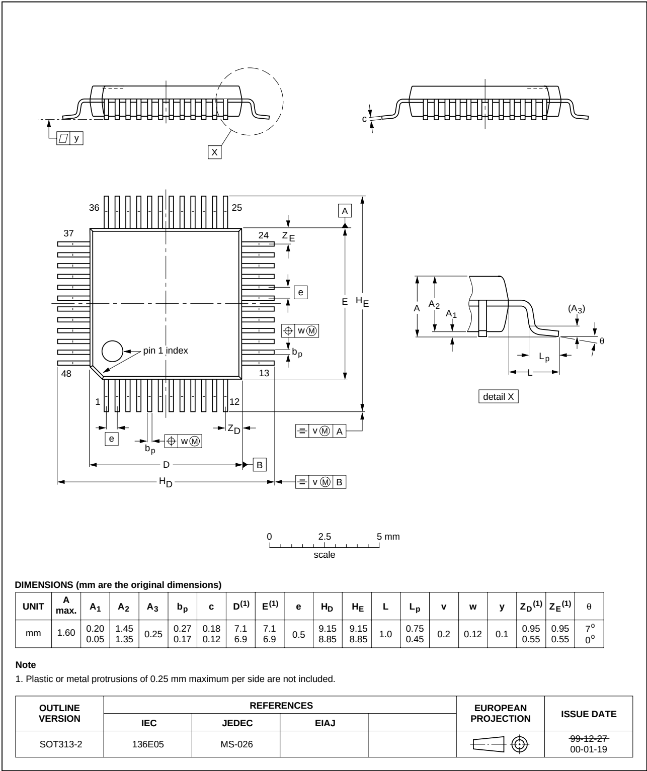
Fig 34. Package outline.
