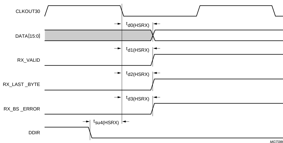
Fig 29. Parallel digital interface timing: high-speed receive.
