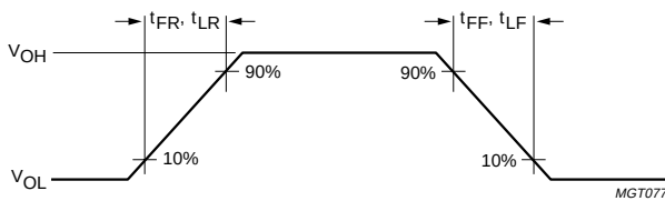
Fig 21. Rise and fall times (FS and LS mode).
