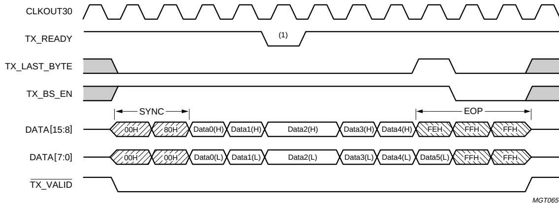
Fig 16. HS receive timing; 5-bytes EOP starting on the high byte.
