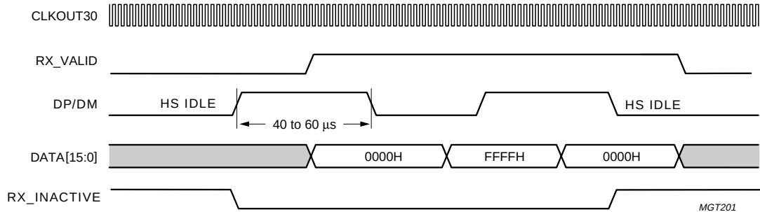
Fig 18. HS chirp receive timing.
