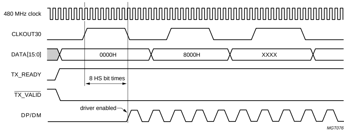
Fig 19. HS transmit path delay.
