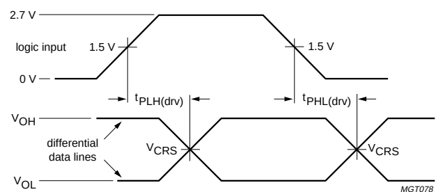
Fig 24. Timing of VO, FSE0 to DP, DM.
