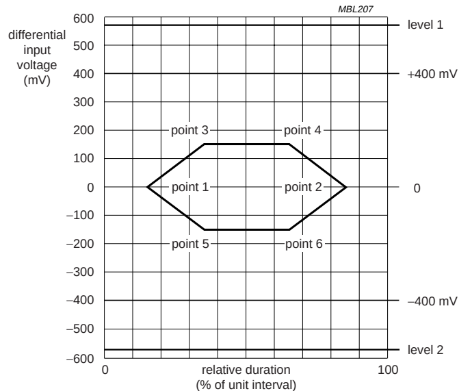
Fig 27. Template 4 eye pattern (receive waveform).
