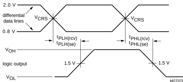
Fig 23. Timing of DP, DM to RCV, VP, VM.
