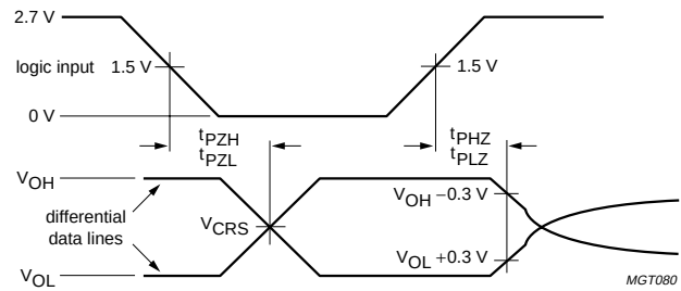
Fig 22. Timing of \overline{OE} to DP, DM.
