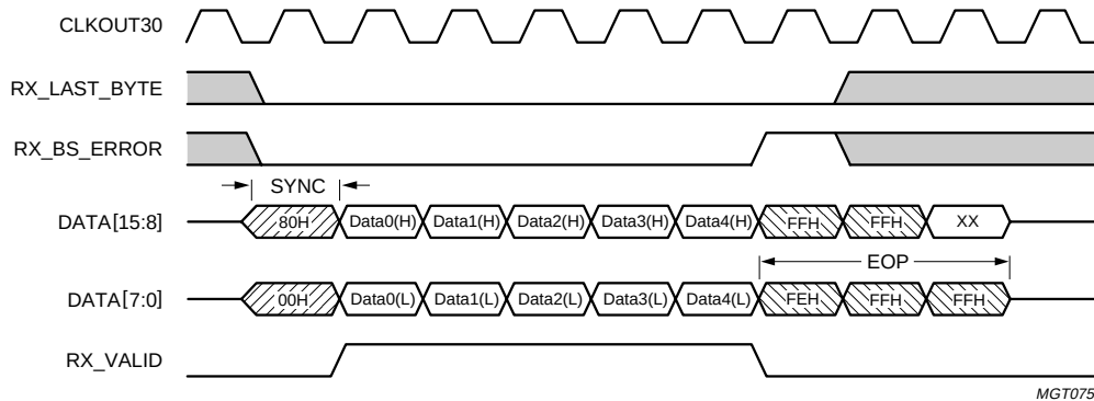
Fig 15. HS receive timing; 5-bytes EOP starting on the low byte.
