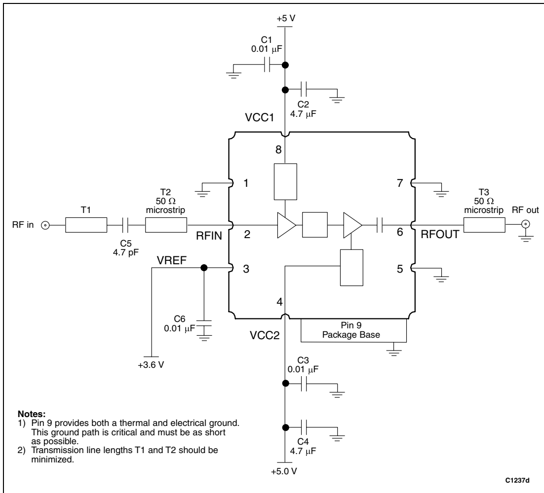
Figure 9. Evaluation Board Schematic, 1700 MHz to 2200 MHz
