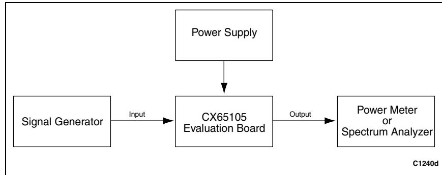
Figure 12. CX65105 Evaluation Board Testing Configuration
