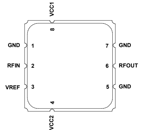
Figure 2. CX65105 Pinout – 8-Pin LCC Package Top View
