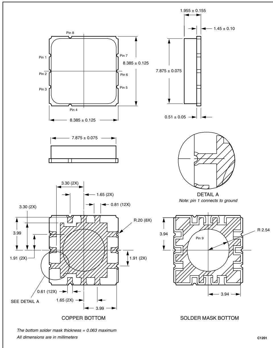
Figure 13. CX65105 8-Pin LCC Package Dimension Drawing
