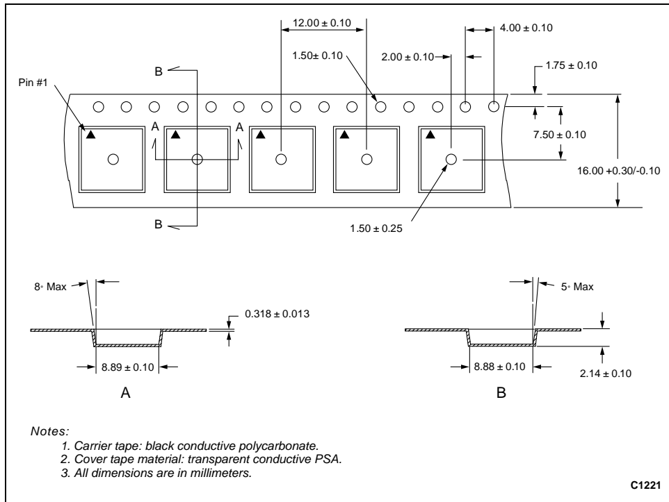
Figure 14. CX65105 8-Pin LCC Tape and Reel Dimensions
