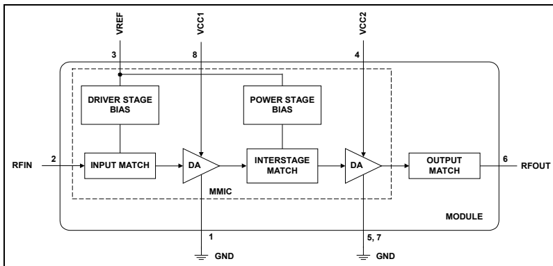
Figure 1. CX65105 Functional Block Diagram
