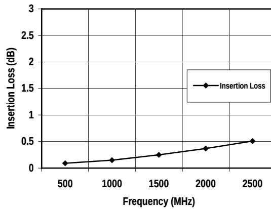
TQ1209 Insertion Loss
