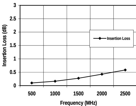
TQ1203 Insertion Loss
