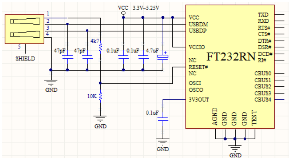
Figure 6.2 Self-Powered Configuration
