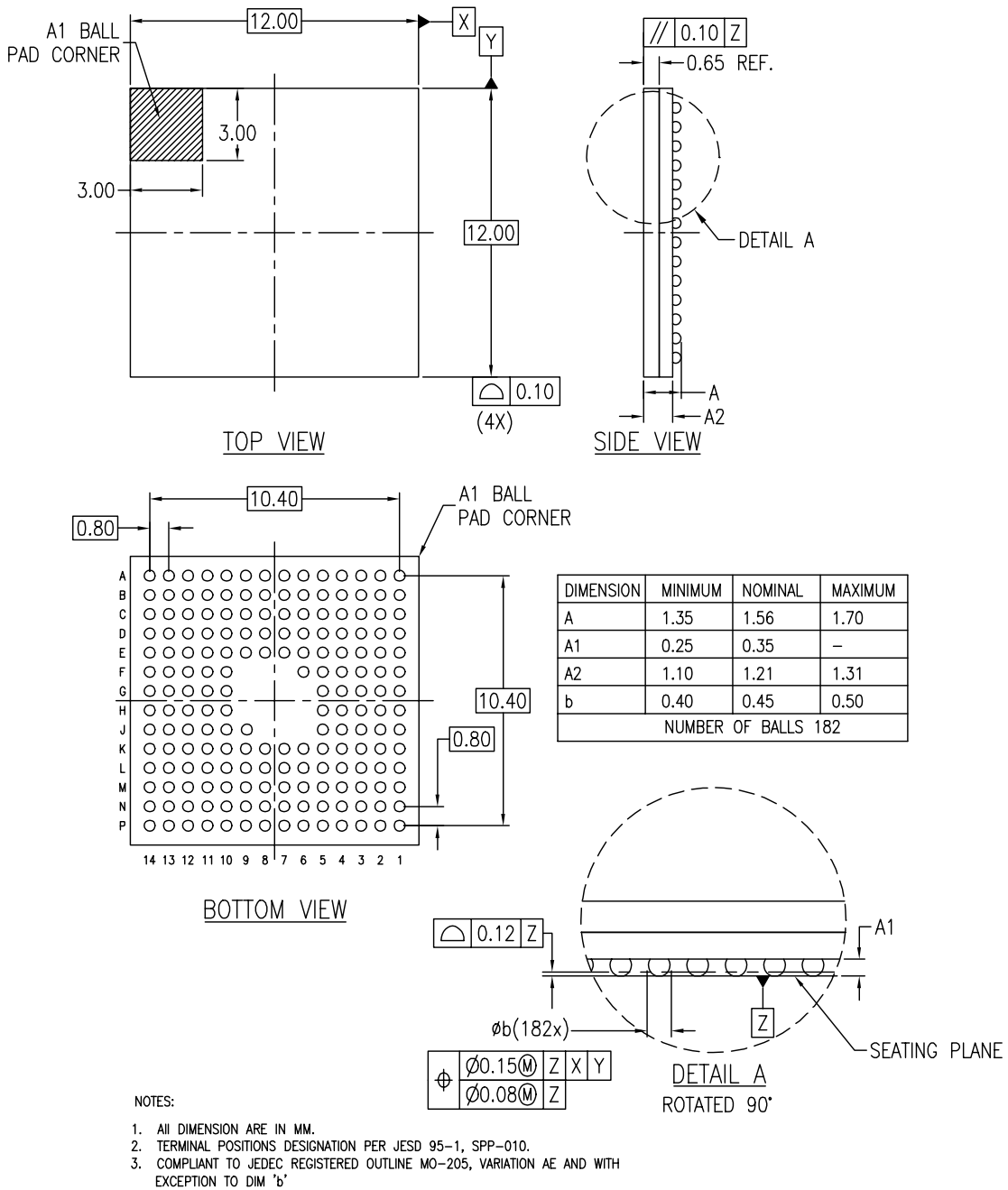
Figure 46. 182-Ball Mini-BGA
