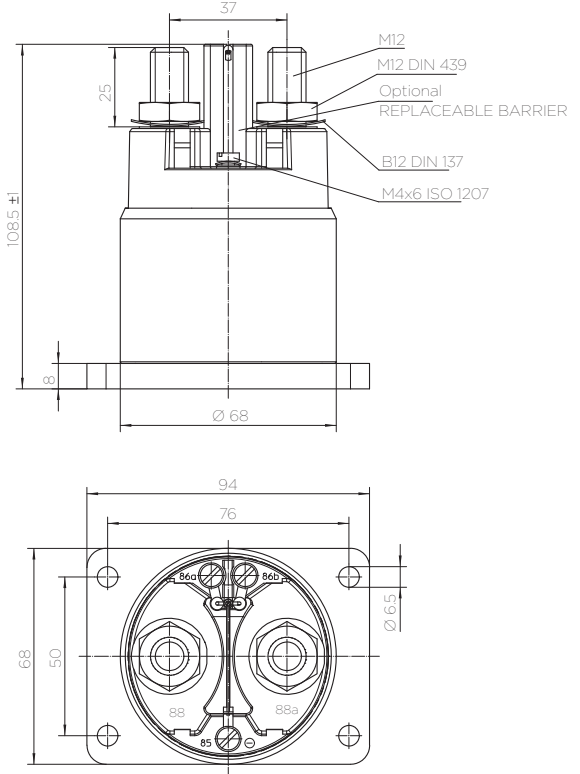
Bottom mounting
