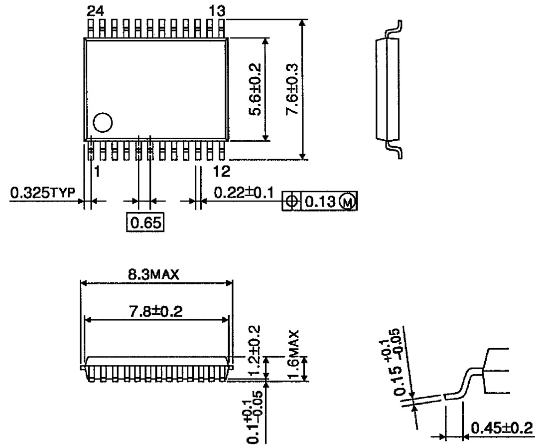
OUTLINE DRAWING SSOP24-P-300-0.65A
