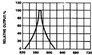
WAVELENGTH ( \lambda )-nm Fig.2 SPECTRAL RESPONSE
