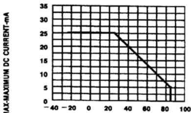
T_A AMBIENT TEMPERATURE ^\circ\text{C} Fig.4 MAXIMUM ALLOWABLE DC CURRENT PER SEGMENT VS. A FUNCTION OF AMBIENT TEMPERATURE.
