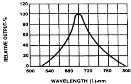
Fig.2 SPECTRAL RESPONSE
