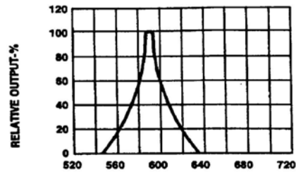
Fig.2 SPECTRAL RESPONSE
