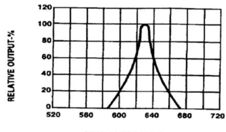
Fig.2 SPECTRAL RESPONSE
