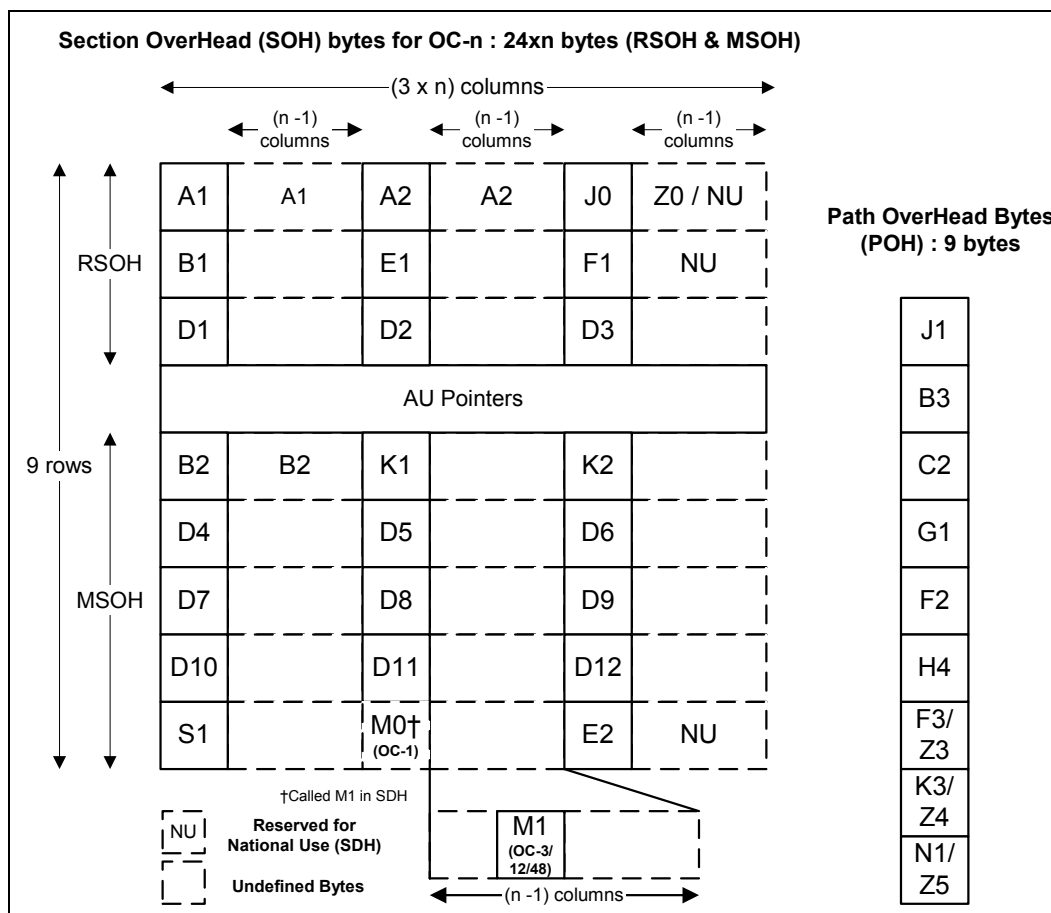
Figure 11. Overhead Bytes for the OC-n
