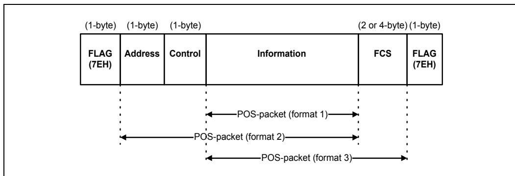
Figure 59. POS-Packet Format
