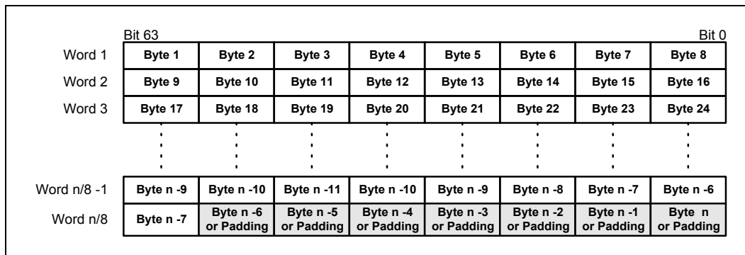
Figure 60. POS-Packet Data Structure Using the 64-Bit UTOPIA Interface
