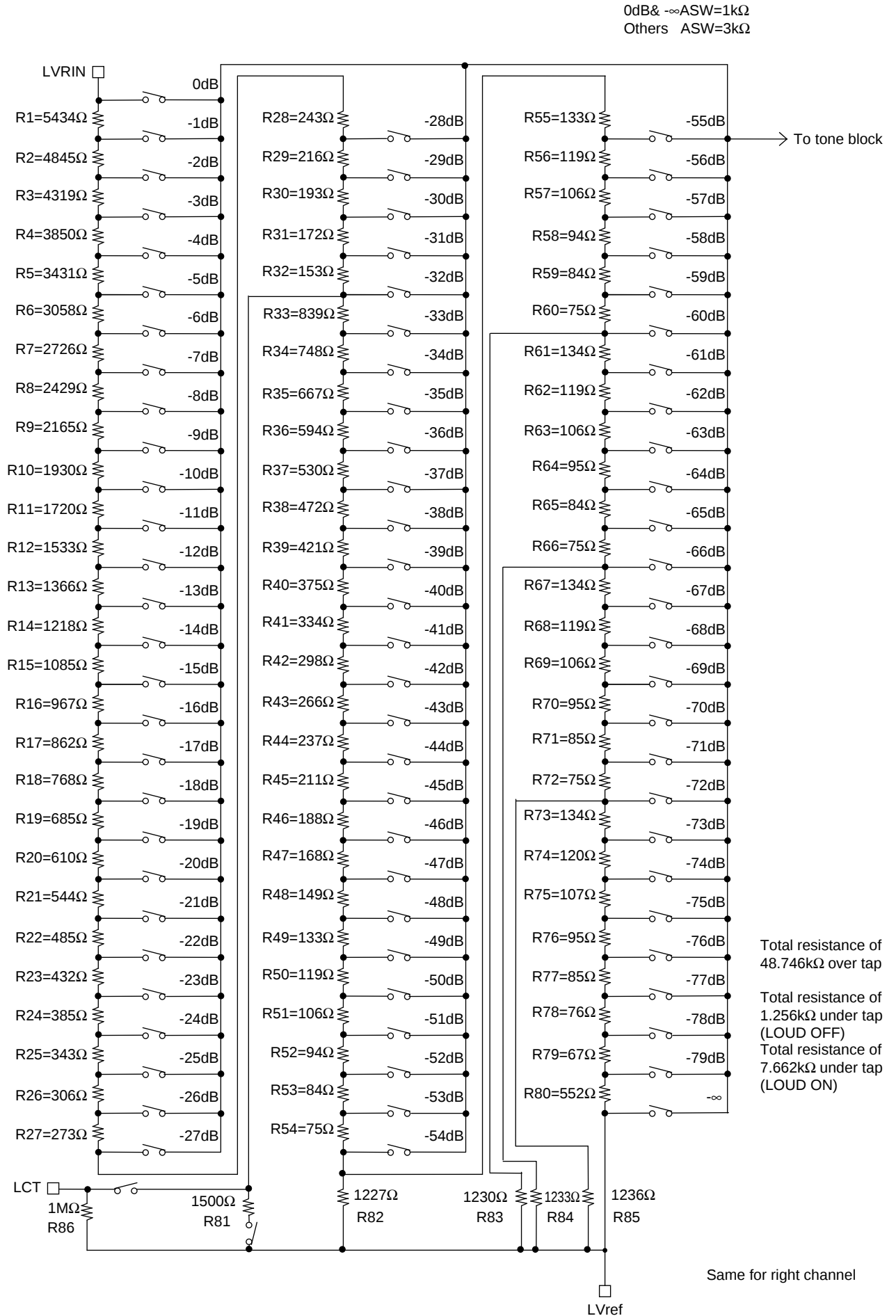
Volume Block Equivalent Circuit Block Diagram
