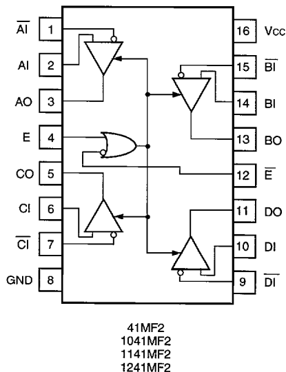
Figure 4-6. 41MF2 Logic Diagram
