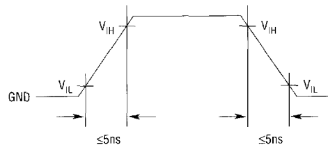
Input Waveforms
