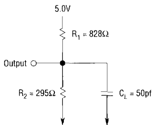
Load Circuit
