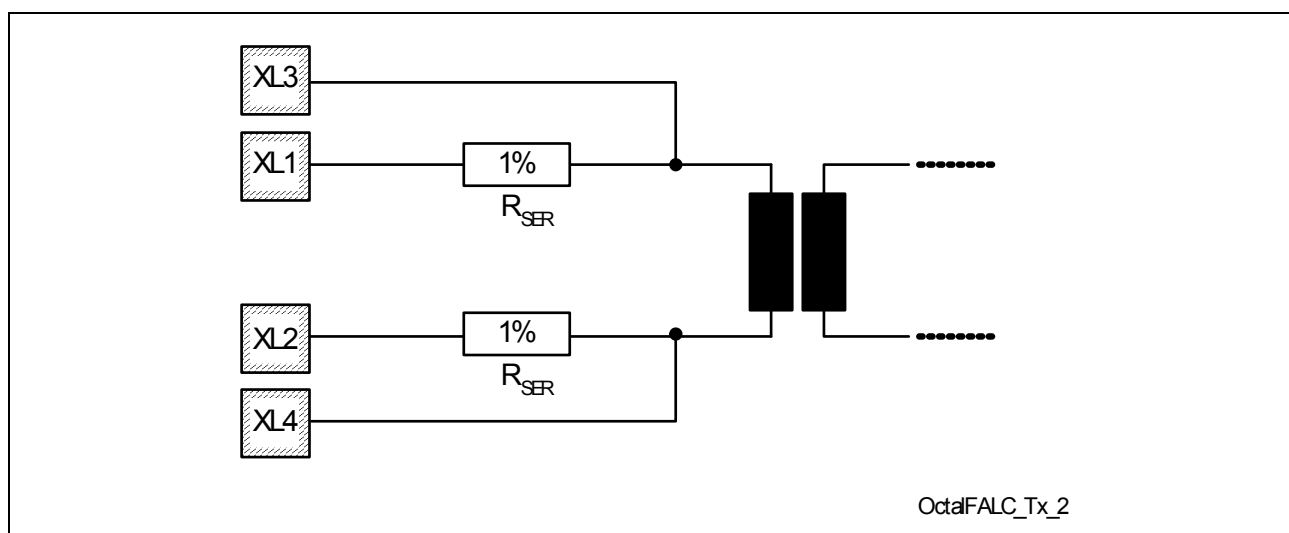
Figure 29 Transmit Impedances
