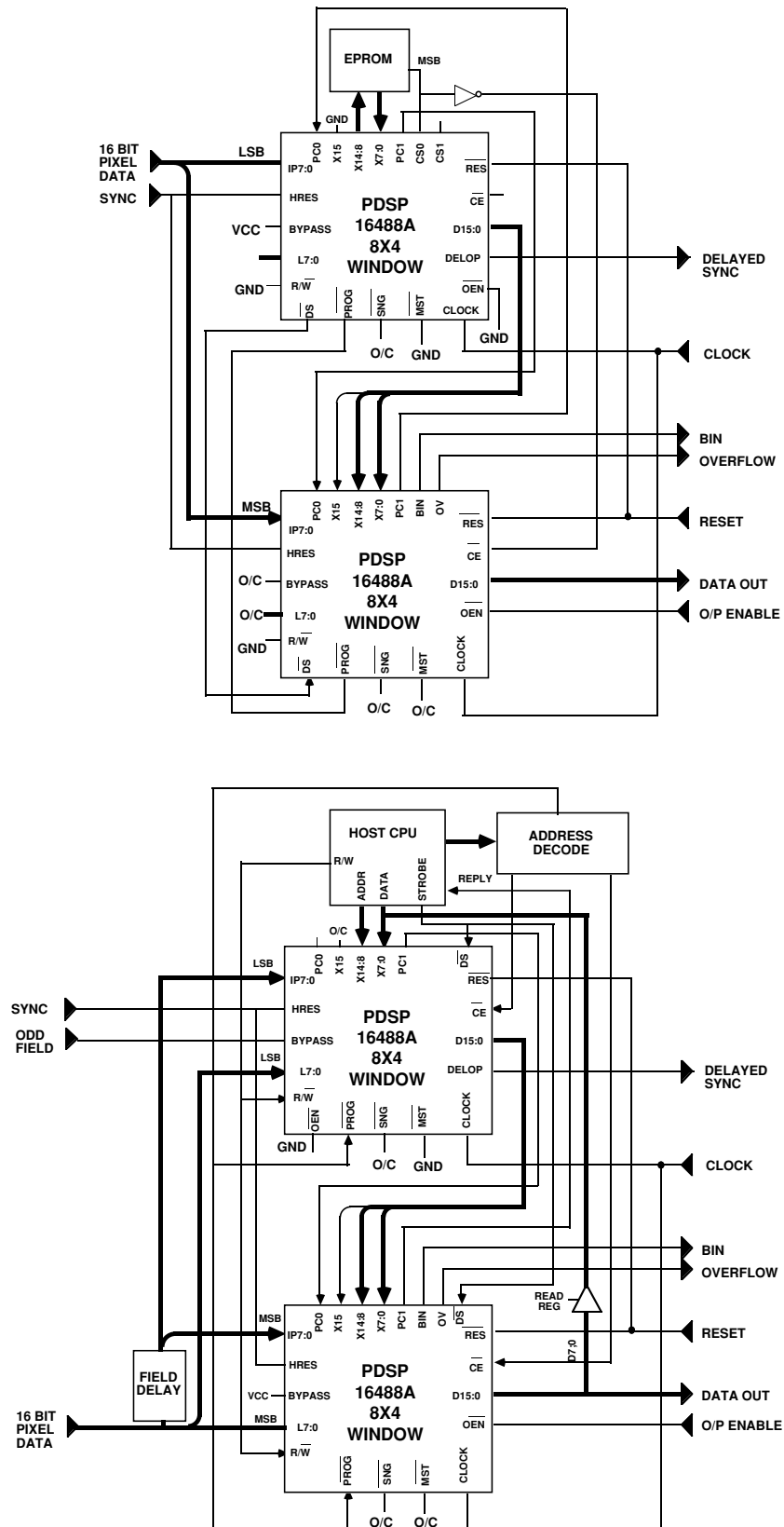
Figure 13. Dual Device 16 Bit Systems.
