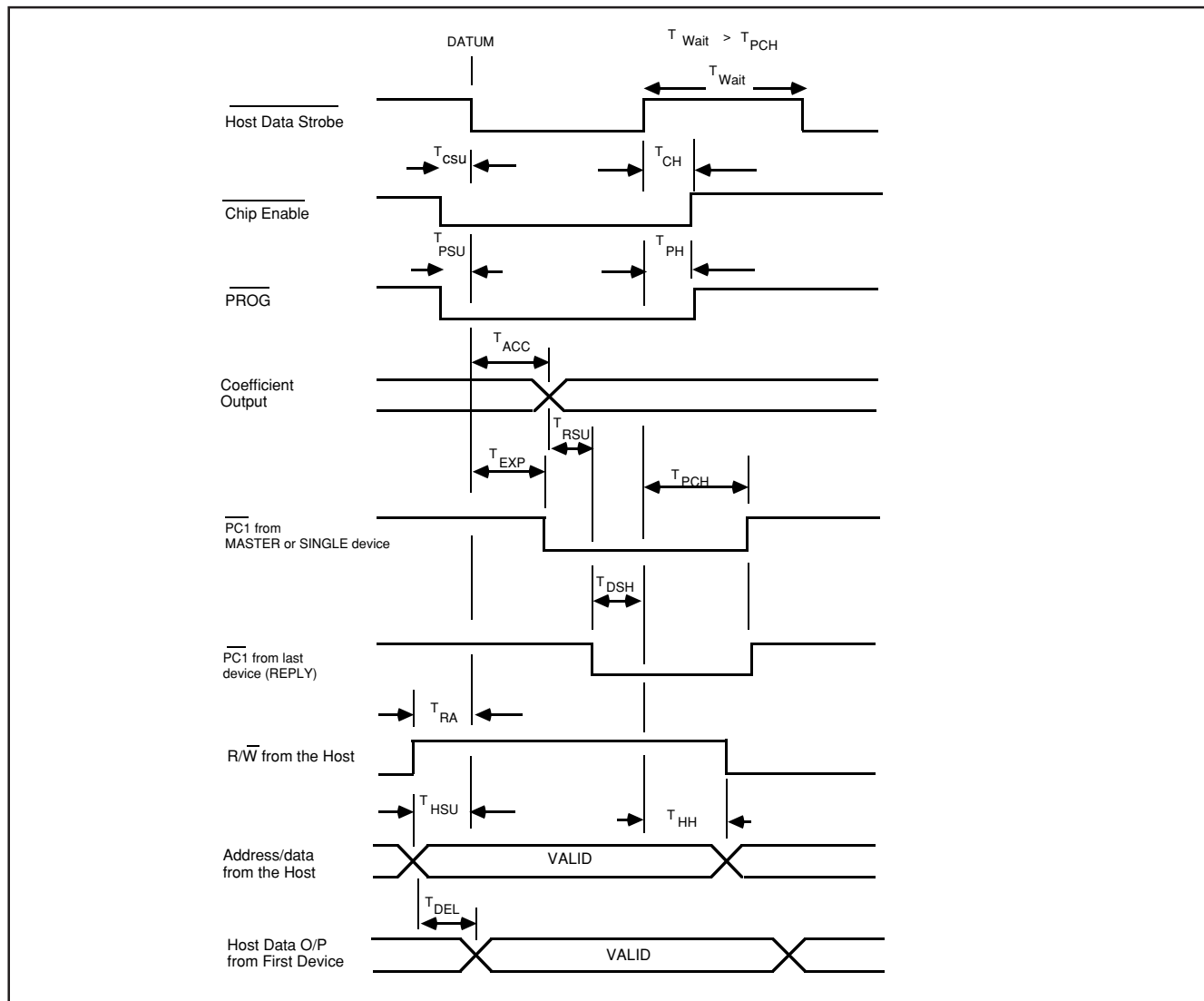
FIG. 8. Host Timing
