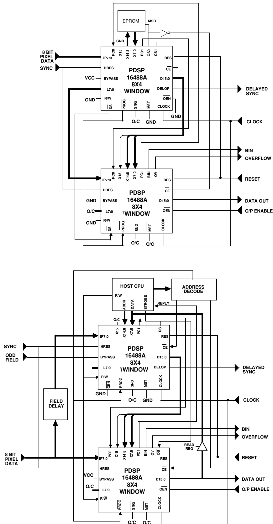
Figure 12. 8 Bit Dual Device Systems
