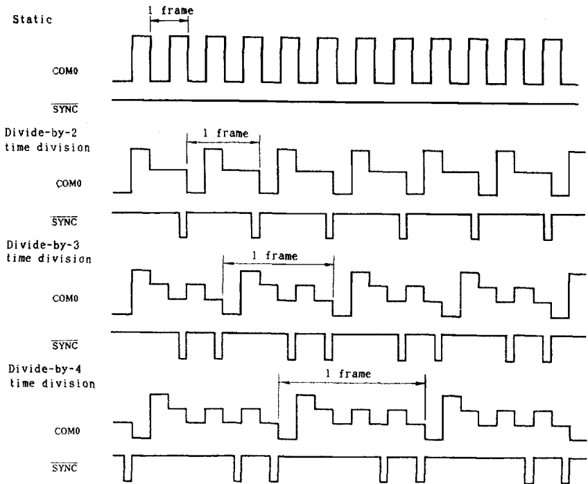
Fig. 2 \overline{\text{SYNC}} Pin Status after Reset ( \overline{\text{RESET}} = 1 )
