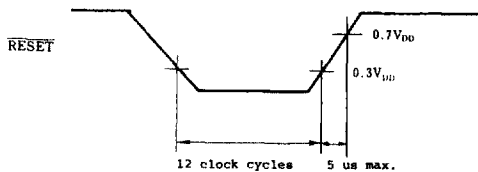
Fig. 12 Reset Signal in Multi-Chip System
