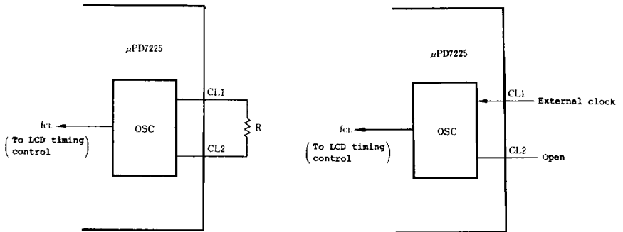
Fig. 11 External Circuit for Clock Oscillation Pins
