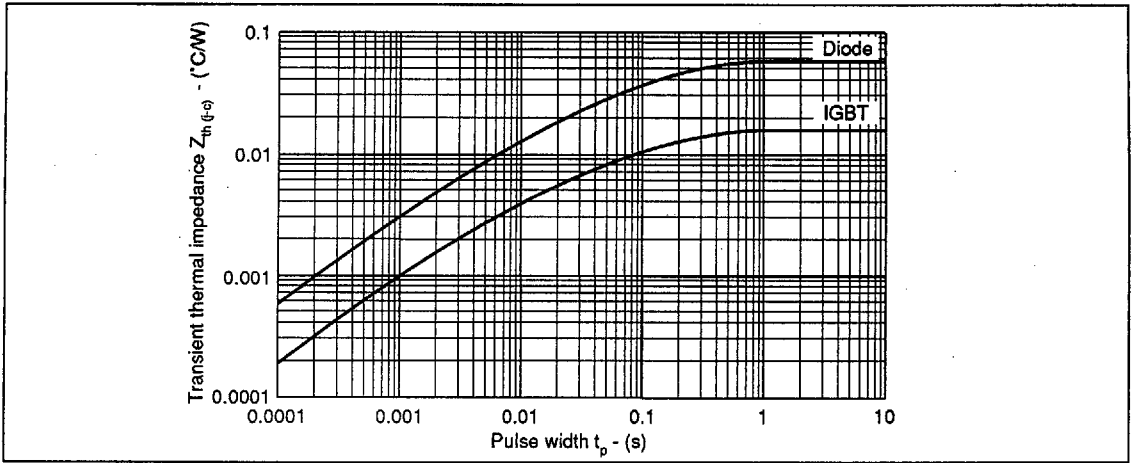
Fig.14 Transient thermal impedance
