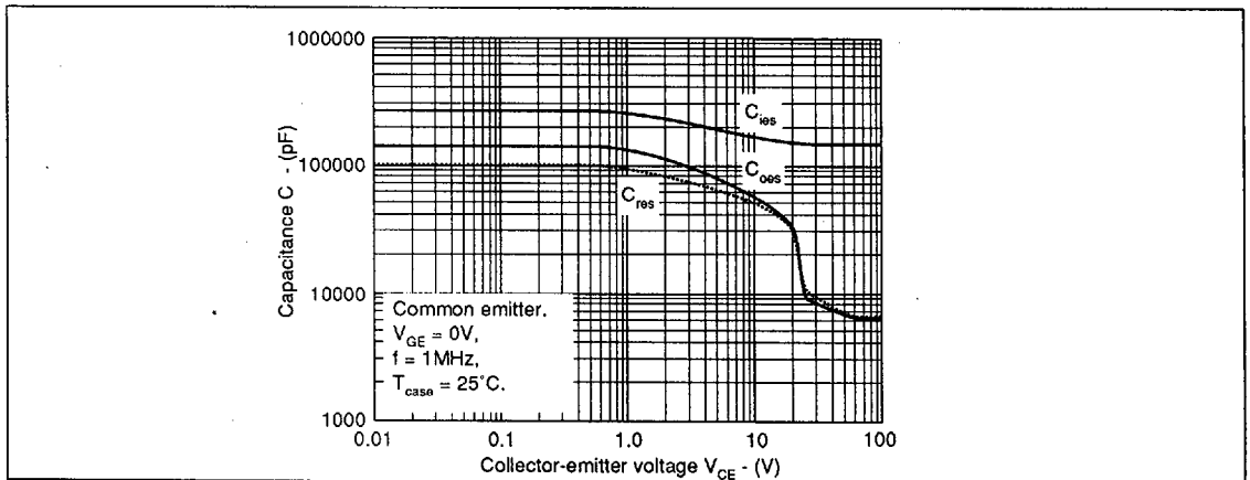
Fig.13 Typical capacitance
