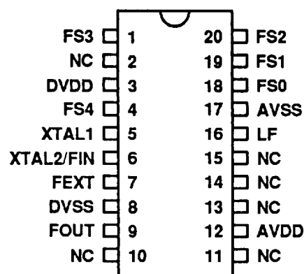
PINOUT DIAGRAM
