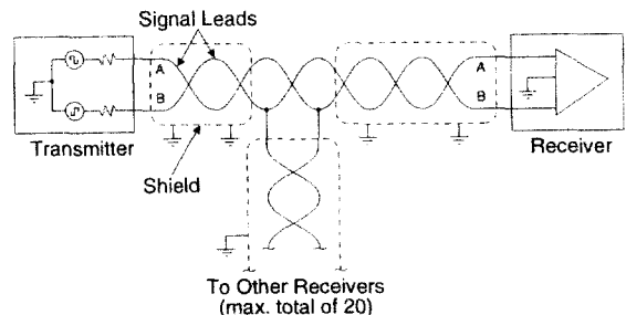
FIGURE 2. GENERALIZED 429 BUS
