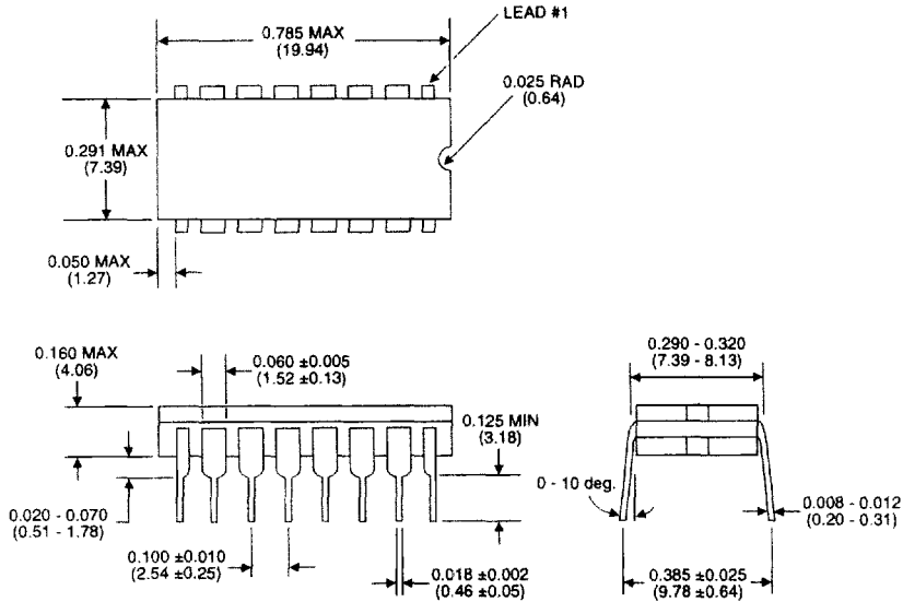
FIGURE 6. DD-03182 CERDIP (JE) MECHANICAL OUTLINE
