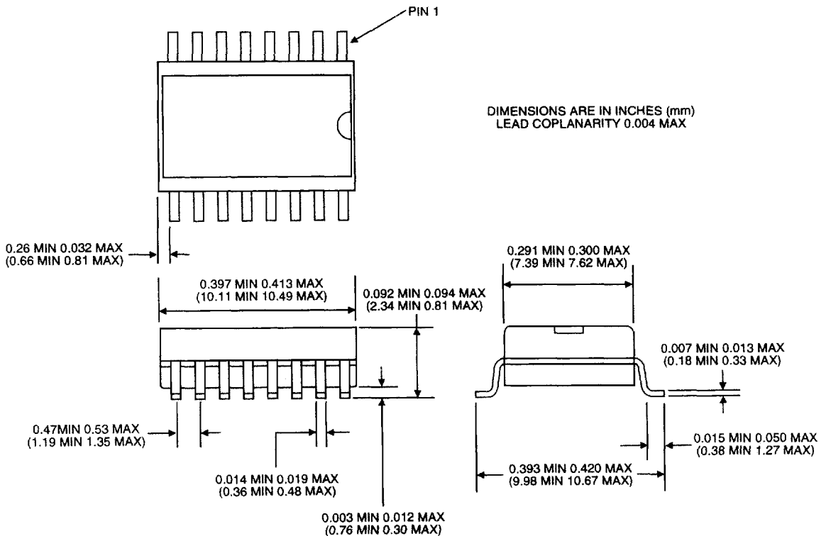
FIGURE 7. DD-03182 SURFACE MOUNT (SOIC) PACKAGE MECHANICAL OUTLINE
